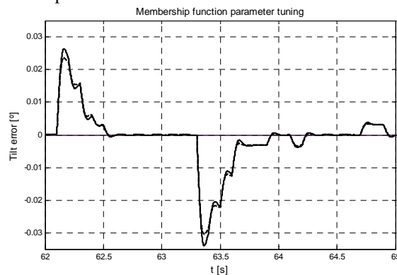
Fig. 4 Error in Tilt angle considering two different sets of membership functions.
