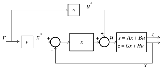
Fig. 3 State Feedback LQ controller with setpoint input
