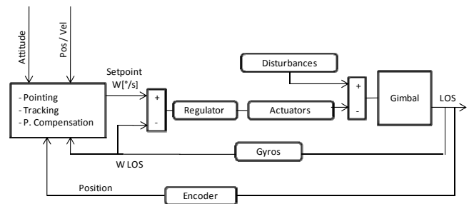
Fig. 2 Stabilized Platform block diagram
