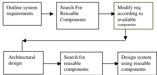
Fig. 1 Software process using reusable artifacts
