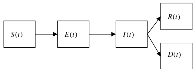
Fig. 2 SEIRD Model
