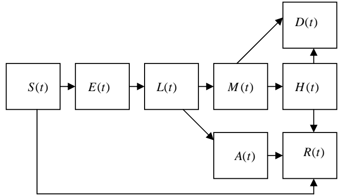
Fig. 4 SELMAHRD model
