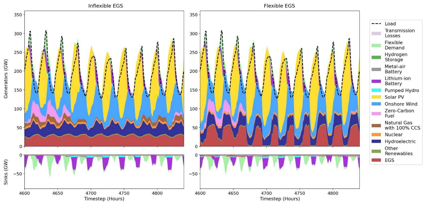
Figure 3: operational snapshots of otherwise identical systems in which EGS is restricted to operating inflexibly (left) or allowed to operate flexibly (right). Flexible EGS complements solar power by shifting generation primarily to nighttime periods.
