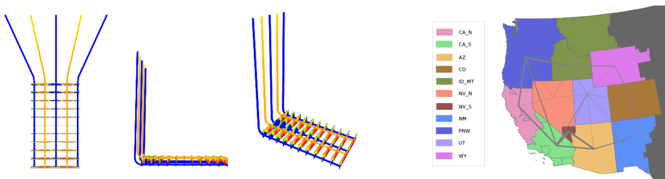
Figure 1: (left) multiple views of the at-scale EGS reservoir design simulated in this work, featuring alternating injection and production wells connected by an engineered fracture network, and (right) a map depicting the network topology used to represent the US Western Interconnection in GenX.
