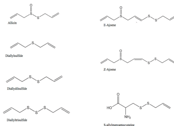
Figure No.10: Allium sativum and its Chemical Structure
