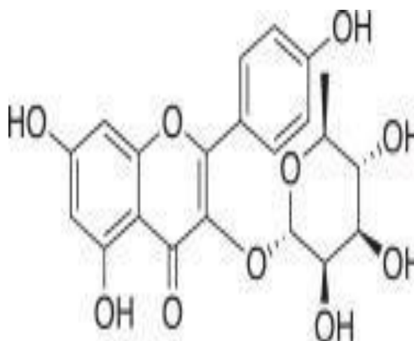
Figure No.15: Phyllanthus Emblica and its Chemical Structure
