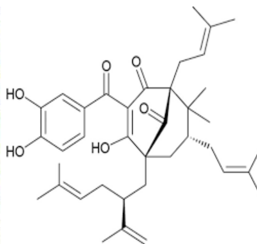
Figure No.11: Garcinia indica linn and its Chemical Structure.
