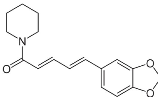
Figure No.19: Piper Nigrum and its Chemical Structure
