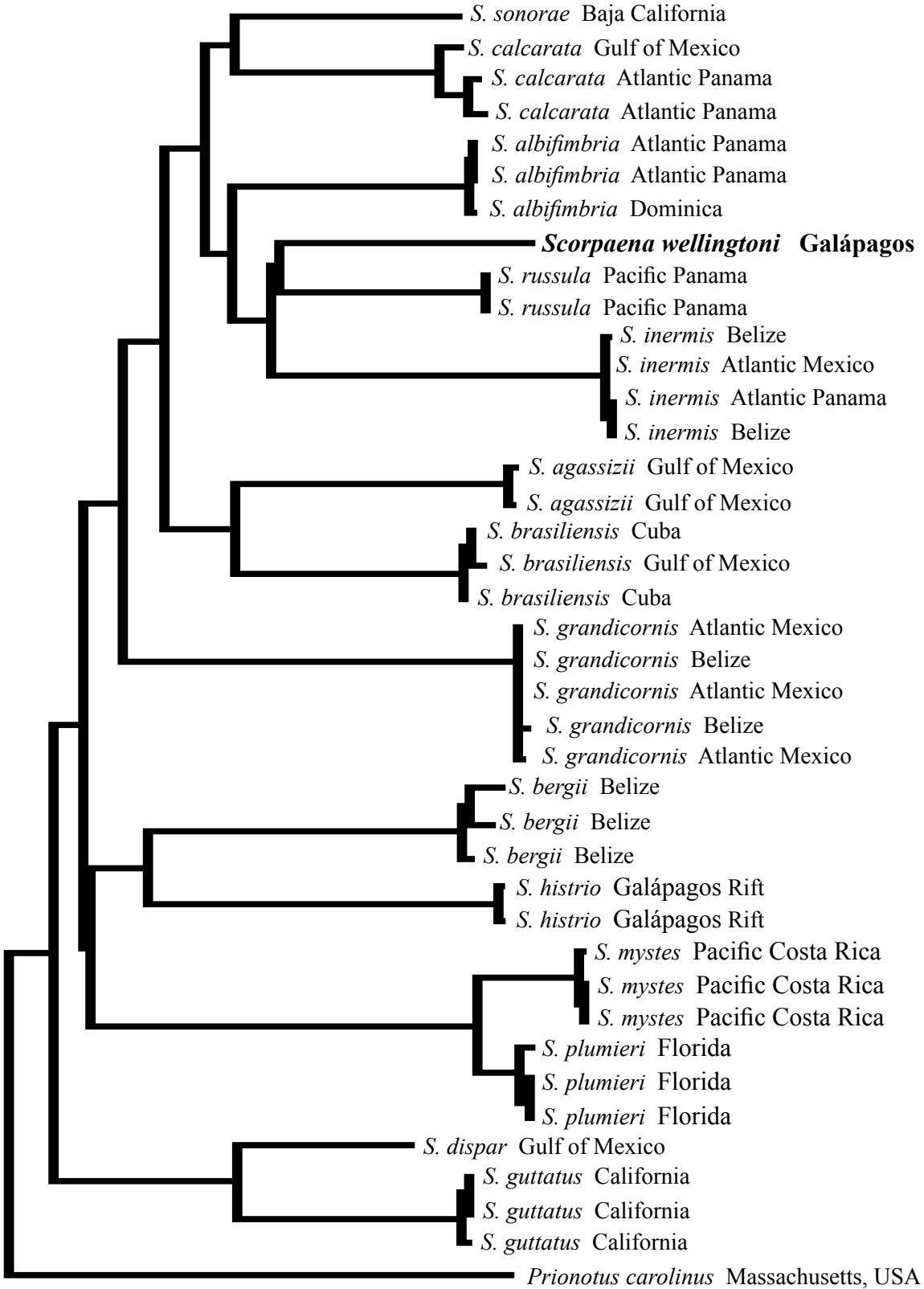
Figure 5. The neighbor-joining phenetic tree based on the COI mtDNA sequences of New World Scorpaena , following the Kimura two-parameter model (K2P) generated by BOLD (Barcode of Life Database). The scale bar at left represents a 2% sequence difference. Collection locations for specimens are indicated and the scorpaeniform Prionotus carolinus is used as an outgroup. GenBank accession numbers and collection data for the sequences in the tree are listed in Appendix 1.
