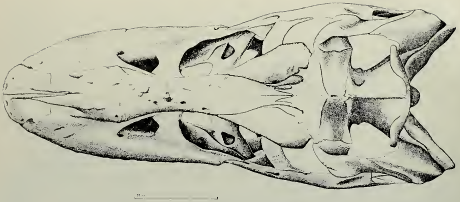
Figure 7— Daspletosaurus torosus , reconstruction of the skull in dorsal aspect, based on NMC 8506.
