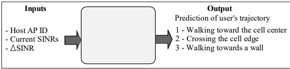
Fig. 5. ML Model for predicting the user's trajectory.
