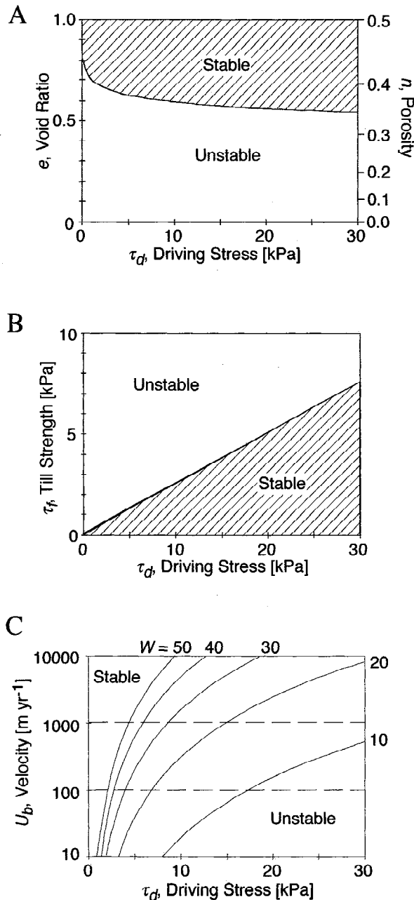
Figure 7. Conditions for the saddle node bifurcation expressed in terms of the three diagnostic variables: (a) void ratio e , (b) till strength \tau_f , and (c) ice stream velocity U_b , given as functions of the two control variables, driving stress \tau_d (equations (13), (14a), and (14b)) and ice stream half width expressed in multiples of ice thickness W . The latter appears only in Figure 7c. Values of the driving stress (0–30 kPa) and of the half-width (10–50) are representative for the West Antarctic ice streams [Bentley, 1987; Shabtaie et al. , 1987]. Diagonal hatching in Figures 7a and 7b marks the fields in which steady state of an ice stream is possible. In Figure 7c, stable states are possible to the left of each of the five curves drawn for different values of W .
