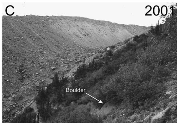
FIGURE 3. Eliot Glacier: (A) termini changes, 1901–2001; (B) view across trough and southeast at right lateral Little Ice Age moraine on 23 July 1901 (H. F. Reid photo in Phillips, 1935); and (C) same view and photo point on 21 August 2001. See photo point on Figure 3A.
