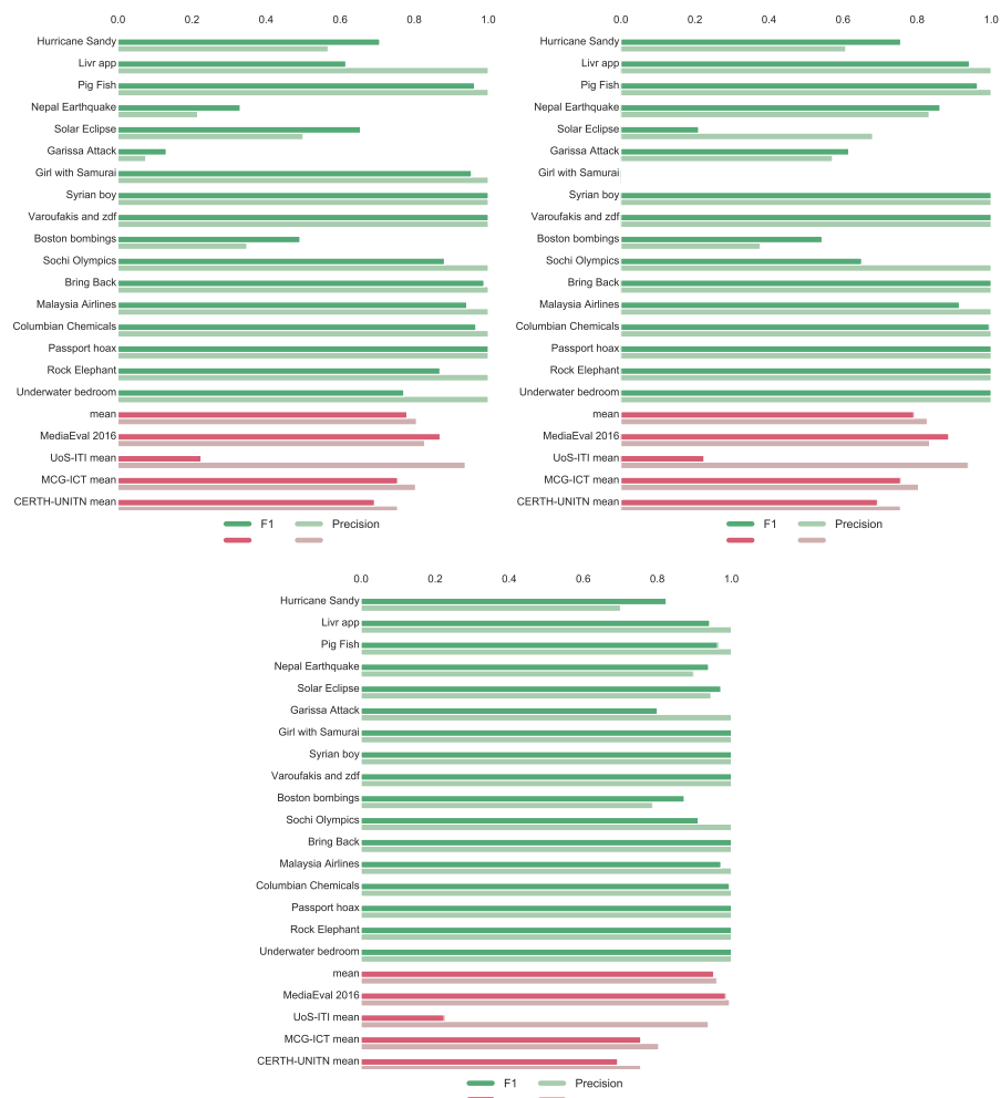
Fig. 11: F1 -scores and Precision of the ENS-MAJ, ENS-HPF and ENS-ORA ensemble methods for dataset#1 , mean score of each method on the dataset of MediaEval '16 and individual mean scores of the approaches.
