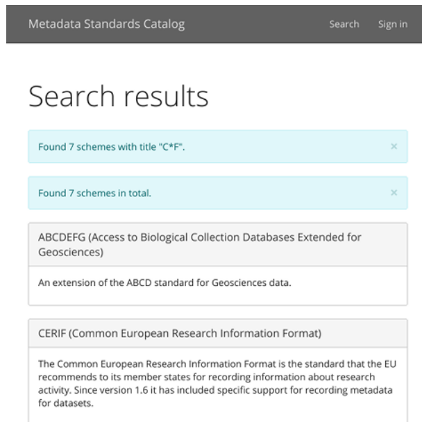
Figure 2.2: Search results
