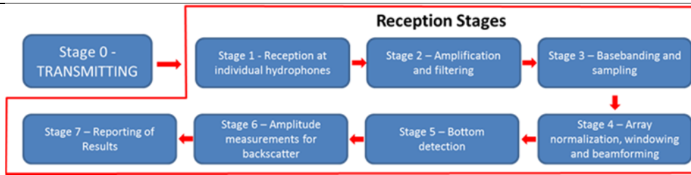
Figure 4-3 An outline of the different stages of backscatter measurement by bathymetric multibeam systems. These stages are generalized somewhat as many differing strategies are employed by different manufacturers (see Section 4.4 for more details).
