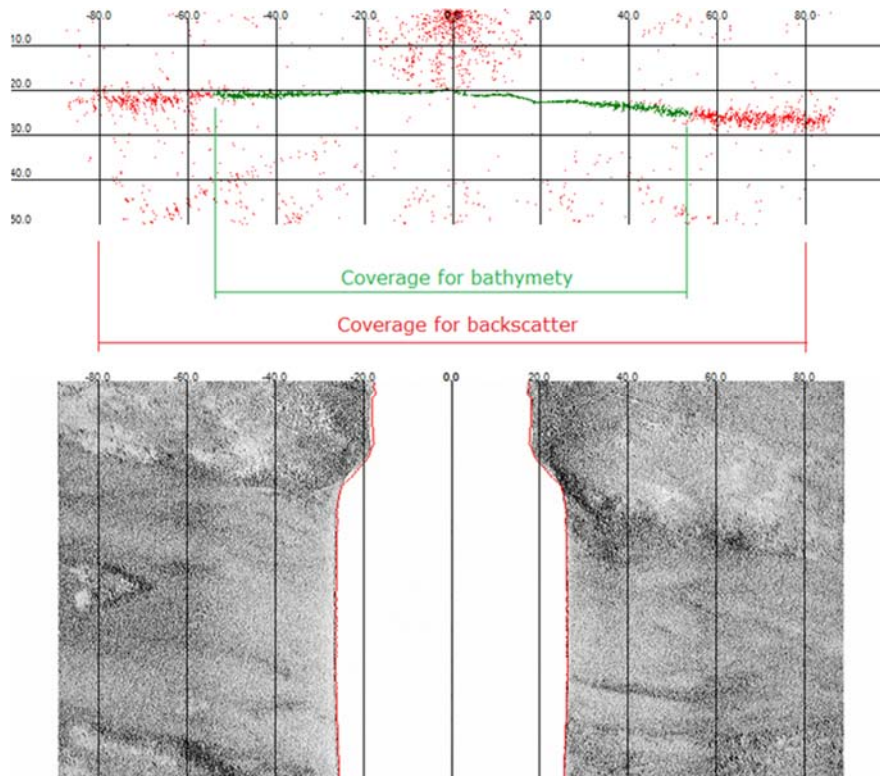
Figure 5-14 Data example from a PMBS, illustrating the difference between effective swath width for bathymetry (green) and backscatter (red).
