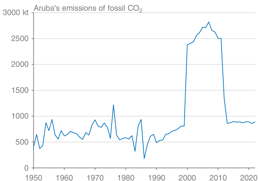
Figure 20: Emissions in Aruba, a Caribbean island, exhibiting an unusual trend.
