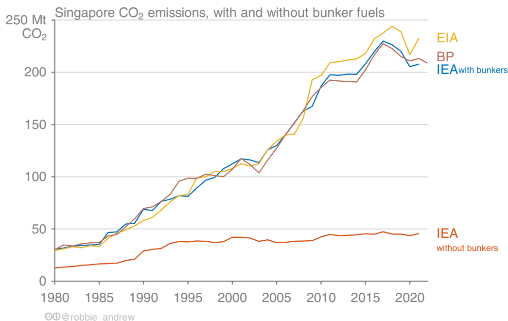
Figure 21: Singapore's CO 2 emissions as reported by several different agencies, demonstrating the very different trend when international bunkers are included.
