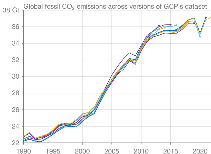
Figure 18: Comparison of global fossil CO 2 emissions from different versions of the GCB dataset. The final data point of each version is always the year before the version number, e.g., the 2021 edition has data through the year 2020 (Y-1).
