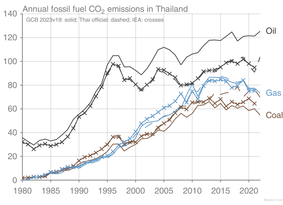
Figure 8: Thailand's emissions of CO 2 from fossil fuels, showing data from Thailand's Ministry of Energy, the IEA, and the previous (internal) edition of the GCB fossil CO 2 dataset.
