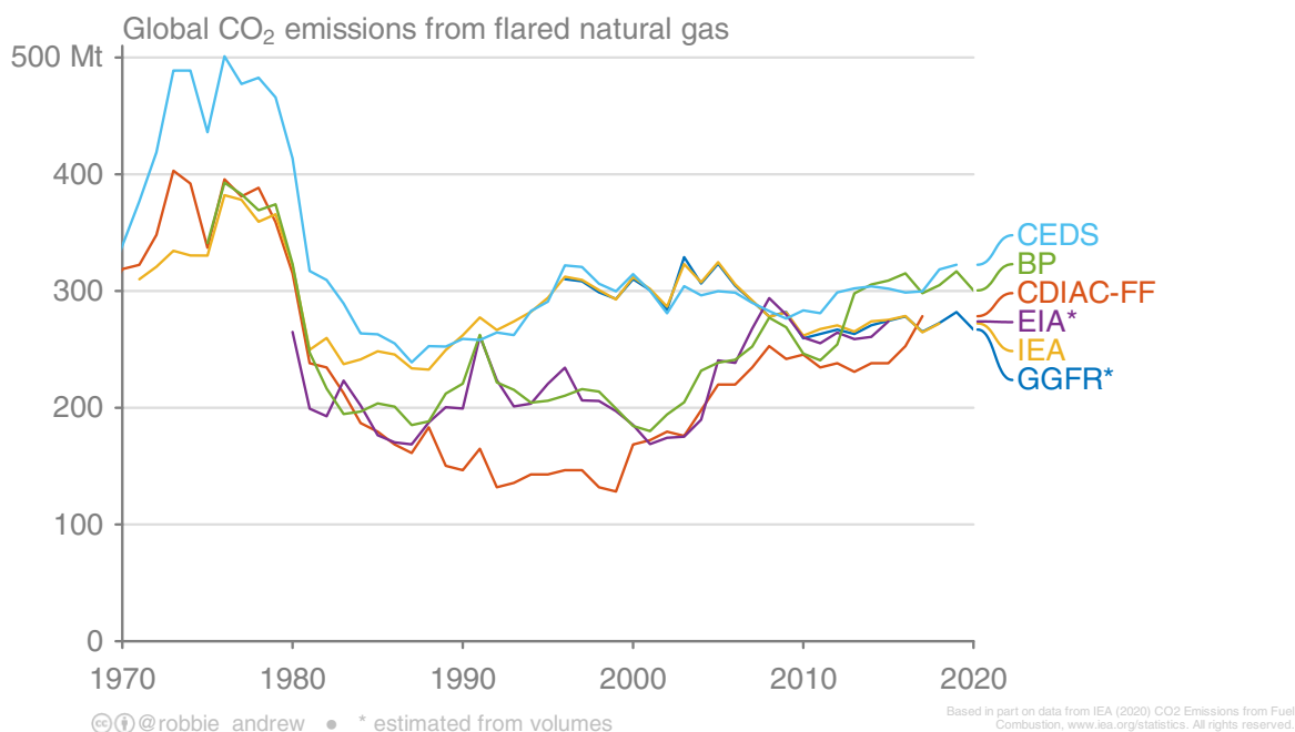
Figure 17: Comparison of estimates of annual global CO 2 emissions from flared natural gas from different sources.
