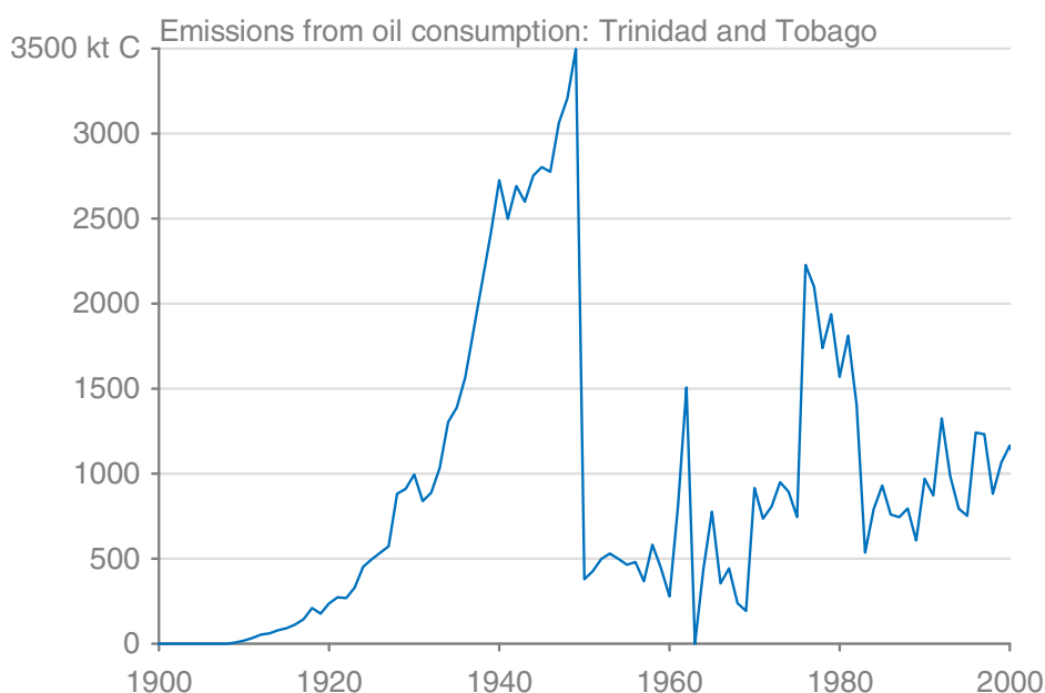
Figure 19: Emissions from oil consumption in Trinidad and Tobago, showing a large discontinuity at 1950 because of a lack of data on sales to bunkers before 1950.
