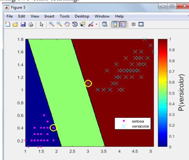
Fig. 10 Plotting of Posterior Probability Regions for SVM Classification Models
