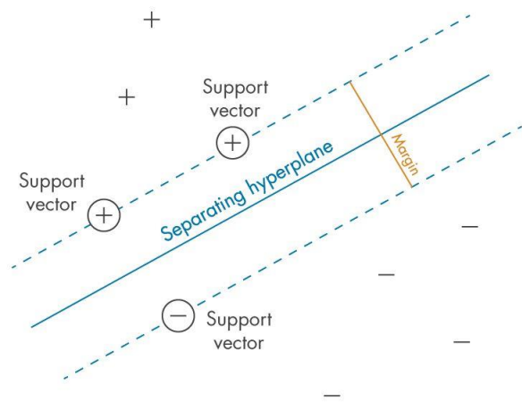
Fig. 1 Separation Hyperplanes
