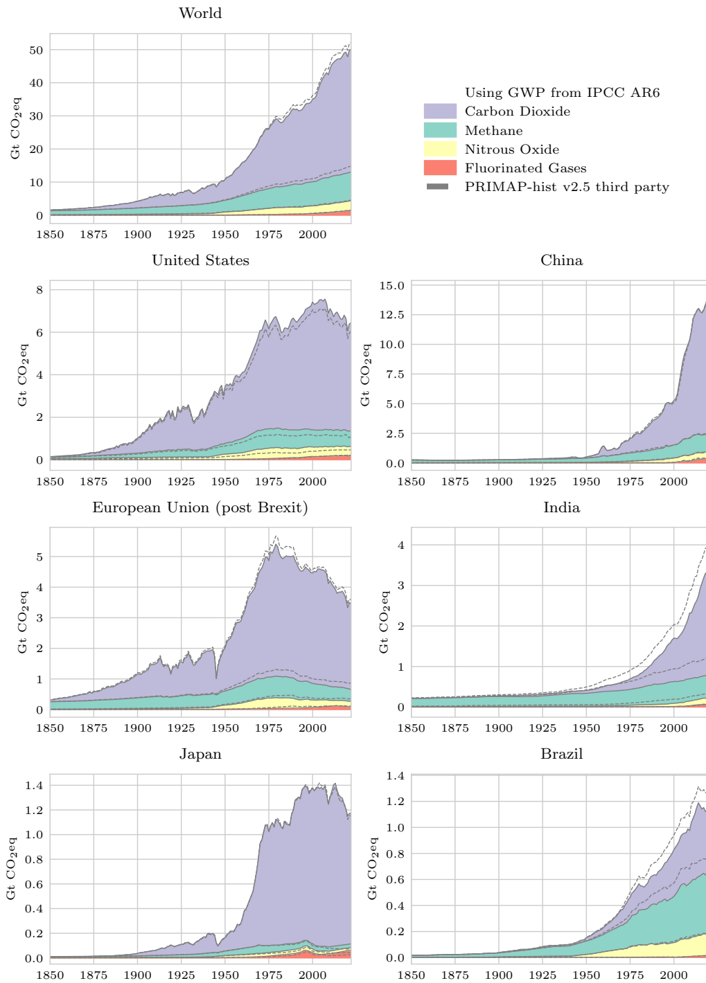
PRIMAP-hist v2.5 country reported priority data by gas for major emitters.
