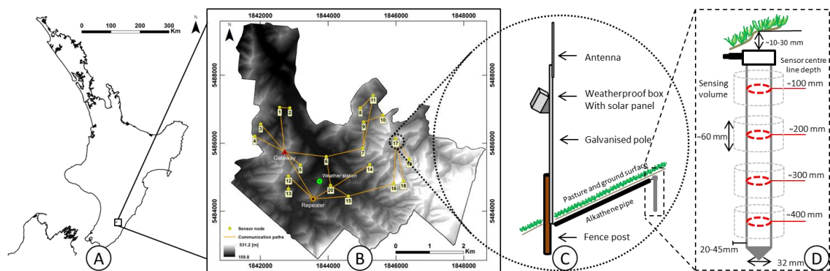
Figure 1. The research area location is shown on (A) and the farm extent is displayed with the WSN architecture and probe IDs on a DEM of the farm (B). The sensor node design is presented in (C) and the configuration of the AquaCheck Subsurface probe with the sensing range on the right (D).
