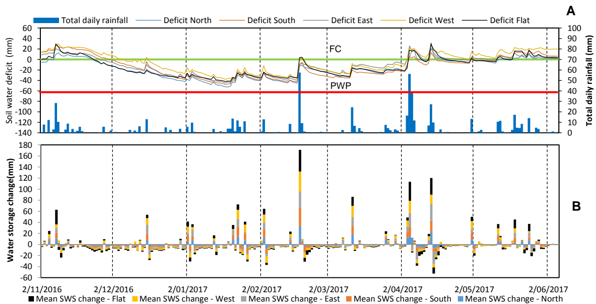
Figure 4. Time series of soil water deficit (A) and daily soil water budget for various aspects (B)
