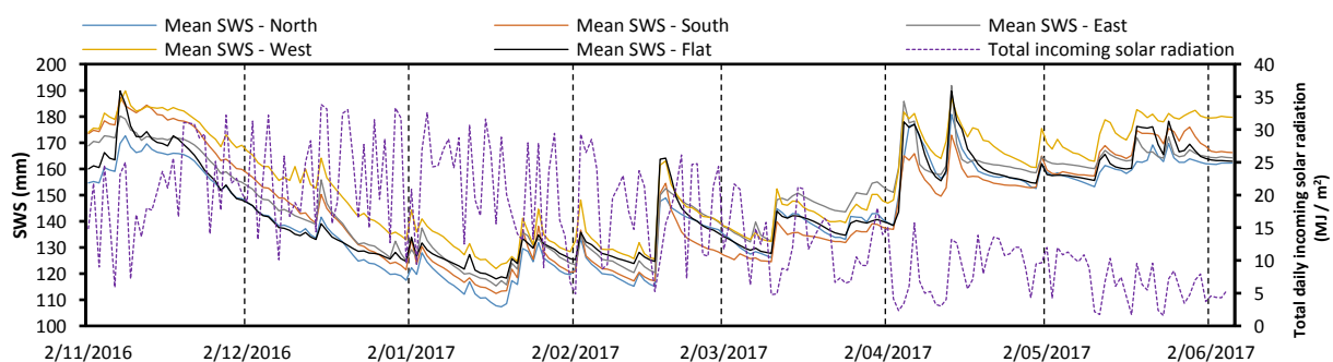
Figure 3. Time series of mean total soil water storage (SWS) for various aspects and daily total incoming solar radiation measured at the weather station's location during a 7 month period
