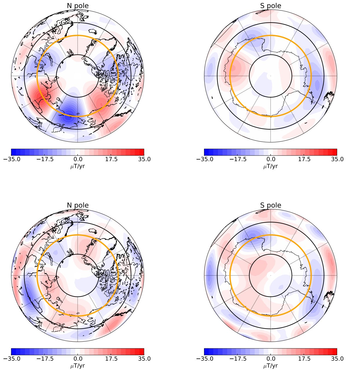
Figure 3: Polar projection view at the CMB of the modelled SV (top row) using a simple jet localised to the tangent cylinder and its residual (bottom row) at epoch 2015. The jet has a maximum azimuthal wavenumber of 1 and a non-dimensional width of \delta = 0.12 . The tangent cylinder is shown in orange, and the lines of 60^\circ and 80^\circ latitude are shown in heavy weight.
