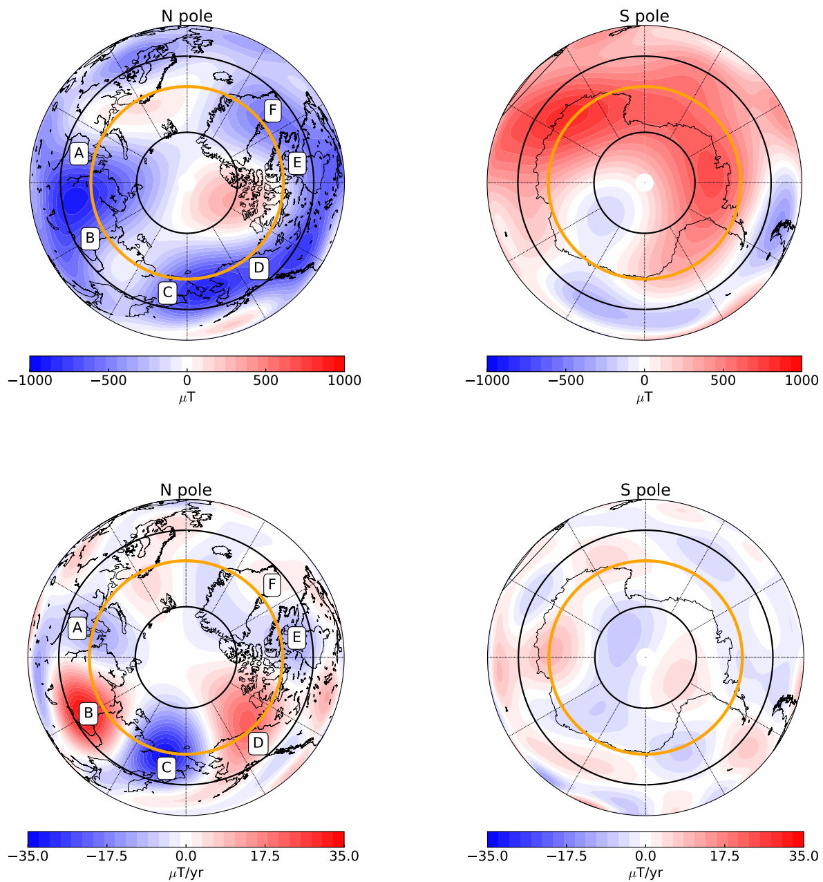
Figure 1: Polar projection view of the main field and secular variation at the CMB from the observation-based field reconstruction CHAOS-6 at epoch 2015. The top row shows the main field to degree 13, while the bottom row shows the SV to degree 16. The tangent cylinder is shown in orange, and the lines of 60^\circ and 80^\circ latitude are shown in heavy weight. Features A–F label patches of SV of alternating sign.
