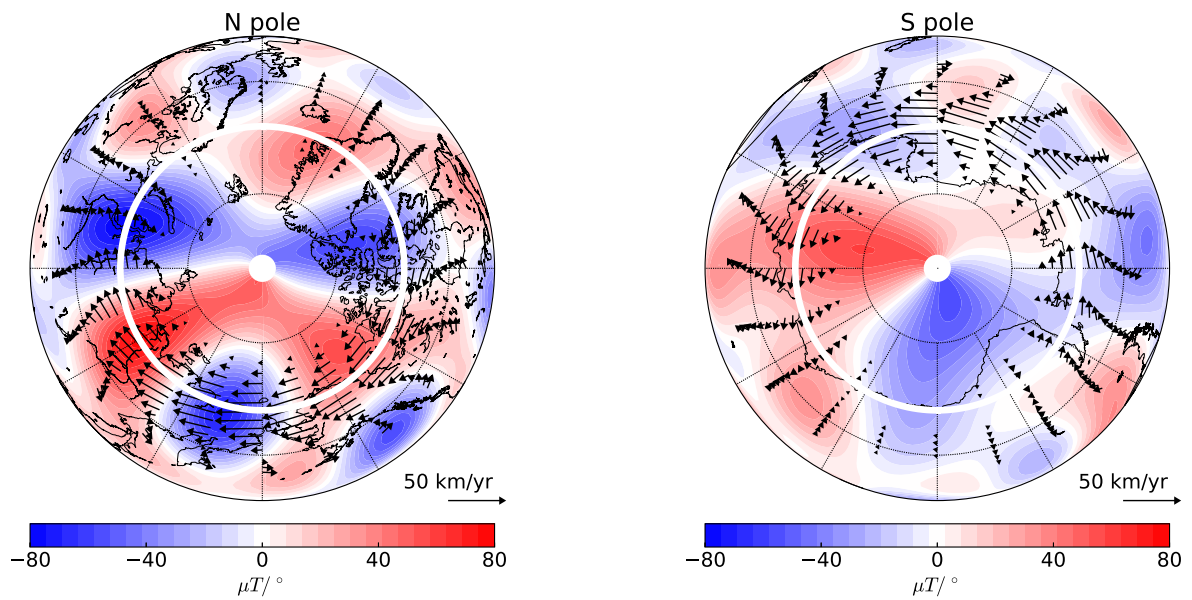
Figure 4: A superposition of the flow direction and magnitude (arrows) and the azimuthal gradient of the radial field (in \mu T/^\circ ) at the CMB using CHAOS-6 at epoch 2015; together these combine to produce the SV when azimuthal-advection dominates. In both plots the line of 180^\circ longitude is at the bottom. In the north, the large gradients in the radial field are advected to produce a strong signature. In the south, weaker gradients in the field where the flow is strong produce comparatively little SV and the jet does not have an observable signature.
