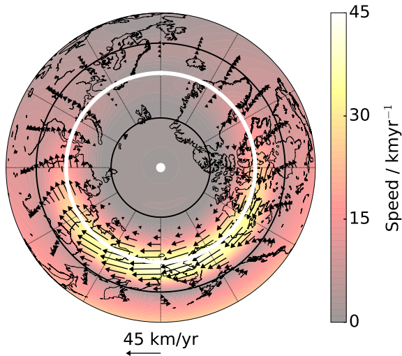
Figure 2: Northern polar view of the flow speed and direction at the CMB of the best fitting high-latitude jet with M = 1 at epoch 2015; the line of 0^\circ longitude is at the top of the figure and the tangent cylinder is marked as a thick white line. The large secular variation under Canada and Siberia can be explained by a cylindrical westwards-directed jet localised on the tangent cylinder reaching a maximum speed of about 40 \text{ kmyr}^{-1} .
