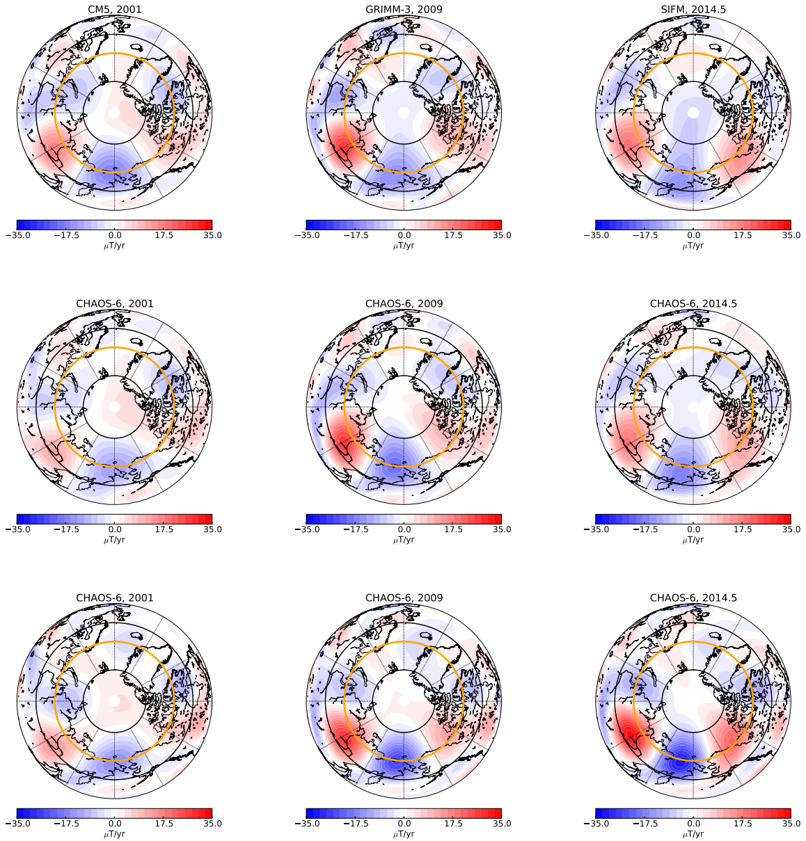
Figure S1: Comparison of SV at the CMB from a variety of models and epochs in a northern polar projection view. In the top row, left: CM5 evaluated to degree 13 in 2001, middle: GRIMM-3, evaluated to degree 14 in 2009, right: SIFM evaluated to degree 11 in 2014.5. Middle row: CHAOS-6 at the same epoch and truncated at the same degree as in the top row. Bottom row: CHAOS-6 at the three epochs but truncated to degree 16. The tangent cylinder is shown in orange, and the lines of 60° and 80° latitude are shown in bold.
