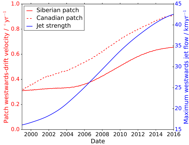
Figure 5: Time-dependence of the jet and drift of high-latitude flux patches. The maximum westwards velocity of the jet (blue, right axis) of maximum wavenumber 1 and width 0.12 has increased in strength over 2000–2016 by a factor of 3. Also shown is the time-dependence of the centre-point of the Siberian (about longitude 100°, solid red) and Canadian (about 200° longitude, dashed red) high-latitude flux patches, which have also increased in westwards speed by a similar factor. The centre-points were determined by the location of the local minimum of radial magnetic field at the CMB according to the CHAOS-6 model to degree 13.
