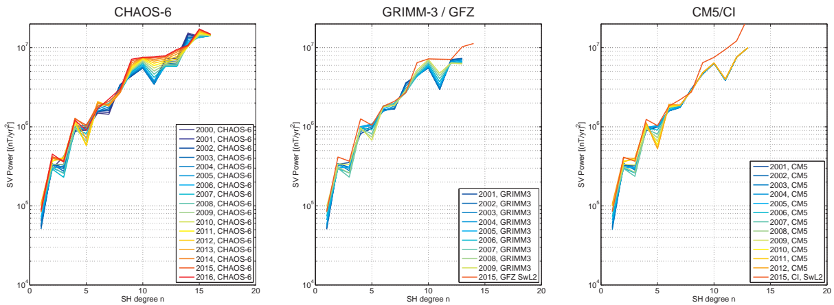
Figure S3: Secular variation power spectra for three different families of models. Both CHAOS-6 and GRIMM/GFZ show time-variation in power at high degree, whereas CM5 shows little variation above degree 6. Thus the strong temporal regularisation used in CM5 does not permit the intensification of the polar SV patches (mainly in degrees 11-13) related to jet acceleration seen in other models.
