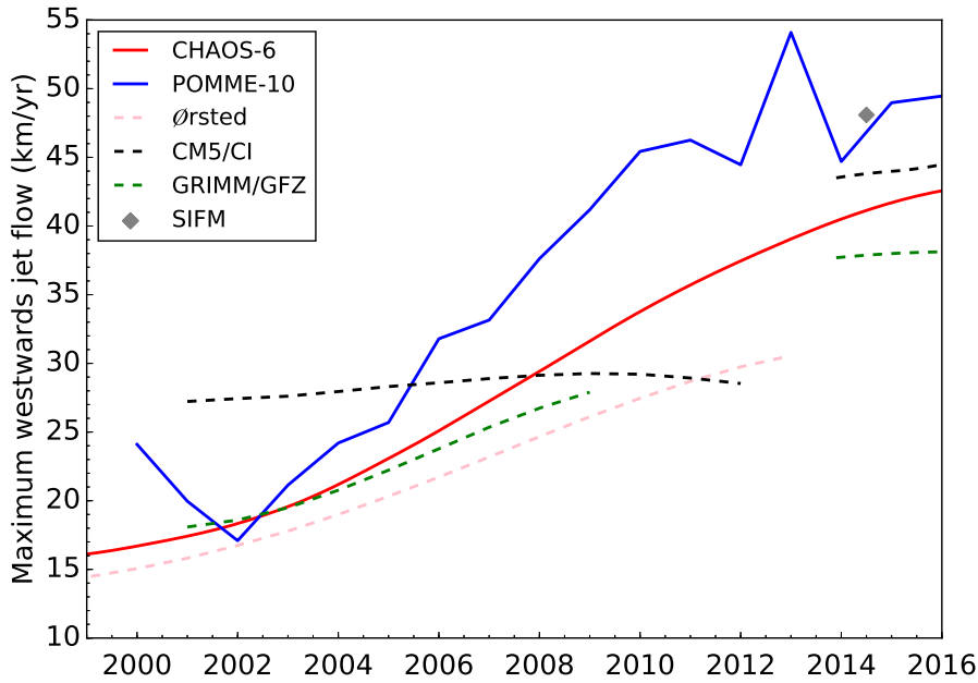
Figure S2: Comparison of maximum westward speeds from the simple jet structure (assuming M = 1 and \delta = 0.12 ) fit to a variety of observational models, whose truncations are described in the methods section of the main text.
