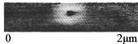
FIG. 4. Current map performed at 4 V on a 2 nm thick \text{SiO}_2 layer after ten RVS from 0 to 5 V.
