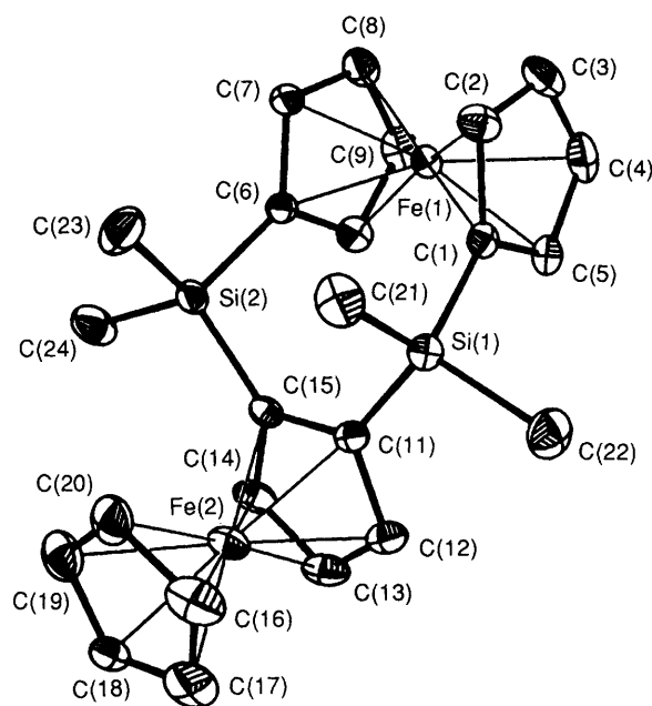
Fig. 2 The molecular structure of 3 (with thermal ellipsoids at the 25% probability level)
