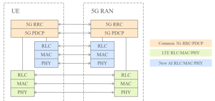
Fig. 3 One possible proposal for control-plane protocol stack that will be investigated in METIS-II.
