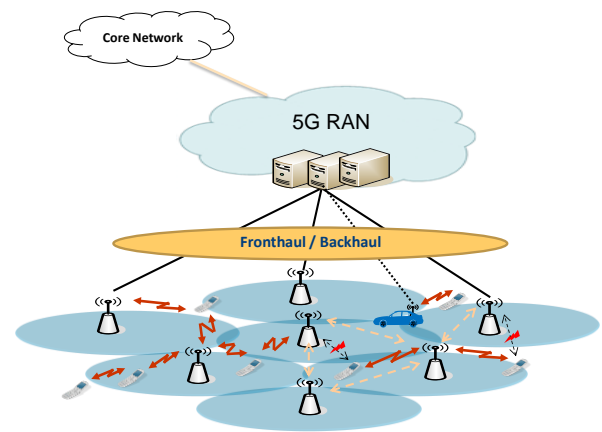
Fig. 2 Inter-cell interference in an UDN scenario.
