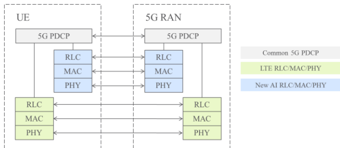
Fig. 4 One possible proposal for user plane protocol stack that will be investigated in METIS-II.
