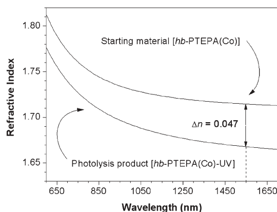
Fig. 2 Refractive indexes of thin films of the cobalt-containing polymer before [ hb -PTEPA(Co)] and after photolysis [ hb -PTEPA(Co)-UV].
