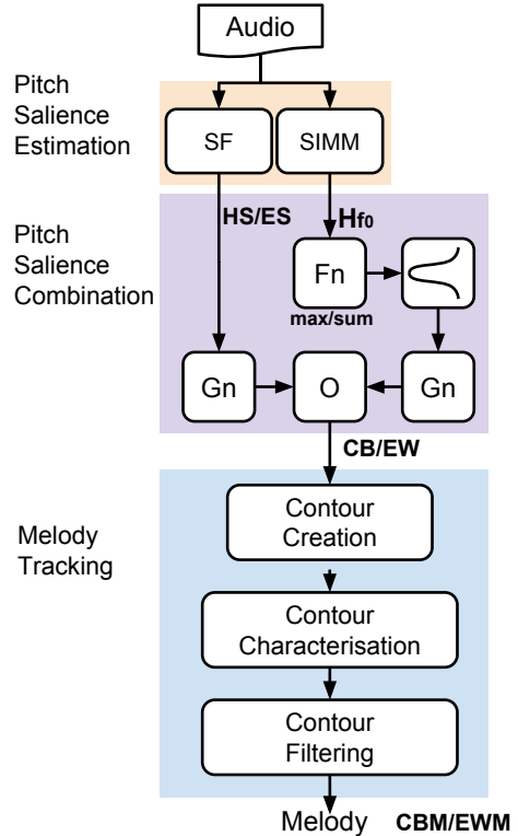
Figure 2: Left: Proposed method schema. SIMM: Smoothed Instantaneous Mixture Model (outputs H_{f_0} ); SF: salience function, either Harmonic Summation (outputs HS) or Energy-based Saliense (outputs ES); Fn: Frame-wise normalisation; Gn: Global normalisation; o: Hadamard product; Gaussian symbol: Gaussian filtering. Combining H_{f_0} with HS we obtain CB. Combining it with ES we obtain EW. CBM and EWM denote the complete melody extraction methods.
