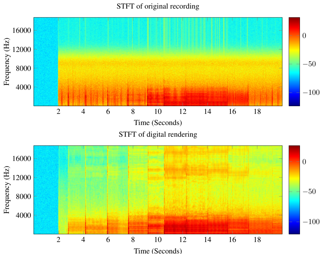
Figure 5. Comparison of STFT plots on a dB scale between the original and re-rendered versions of Musical Stairs , using an FFT size of 4096 and a hop size of 1024
