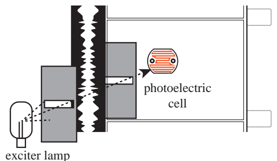
Figure 1. Diagram of the optical sound head
