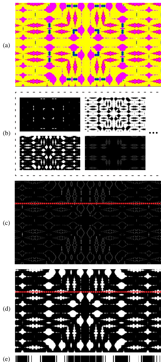
Figure 6. Image processing stages in No-Input Pixels . The frame (a) is filtered into eight color maps (b). Each map is analyzed using horizontal and vertical edge detection (c), and the busiest row and column (represented by the red line) are selected from the original map (d). The selected rows and columns are output (e) and sent to the virtual optical sound head.
