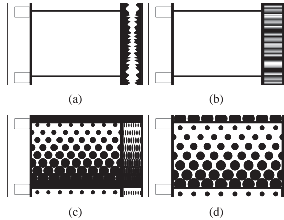
Figure 2. Examples of optical soundtracks: (a) variable area, (b) variable density, (c) soundtrack made from camera images, (d) Super16 images extending onto soundtrack area
