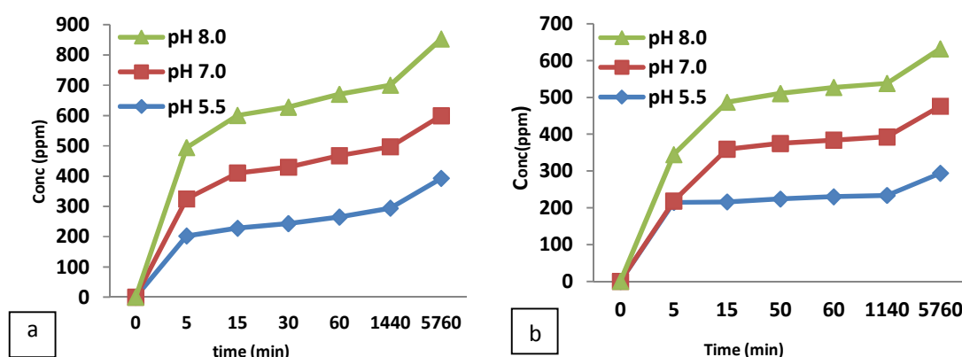
Fig. 6. Concentration of pendimethalin released from (a) 0.8% and (b) 0.3% loaded CuCtsNPs
