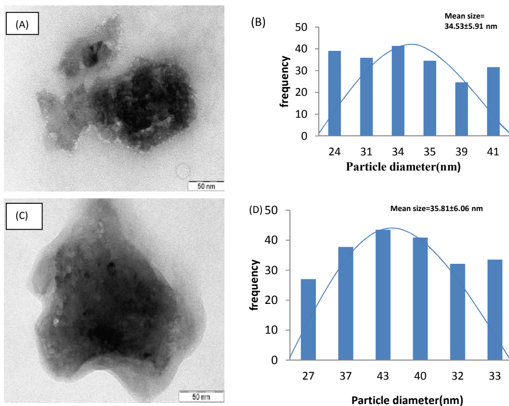
Fig. 4. TEM images of the synthesized CuCtsNPs and Pend-CuCtsNPs (A and C) and their particle size distribution histograms (B and D)
