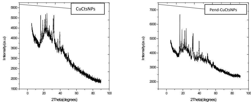
Fig. 3. PXRD Diffractogram of CuCtsNPs and Pend-CuCtsNPs
