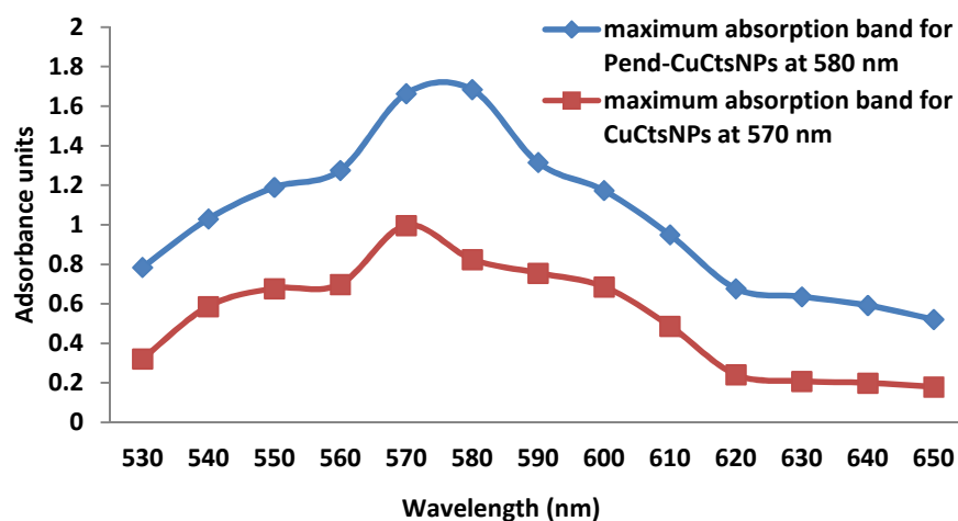
Fig. 1. UV-visible spectral of CuCtsNPs and Pend-CuCtsNPs
