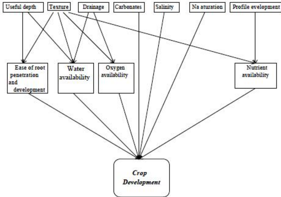
Fig. 5. Direct and indirect effects of the selected soil characteristics on crop production
