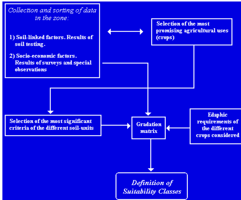
Fig. 4. Diagram showing the methodology followed in Almgren model
