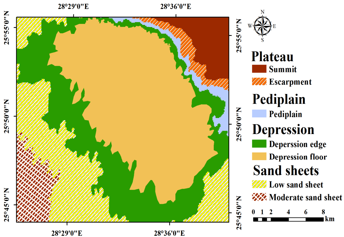
Fig. 6. Landforms of the studied area
