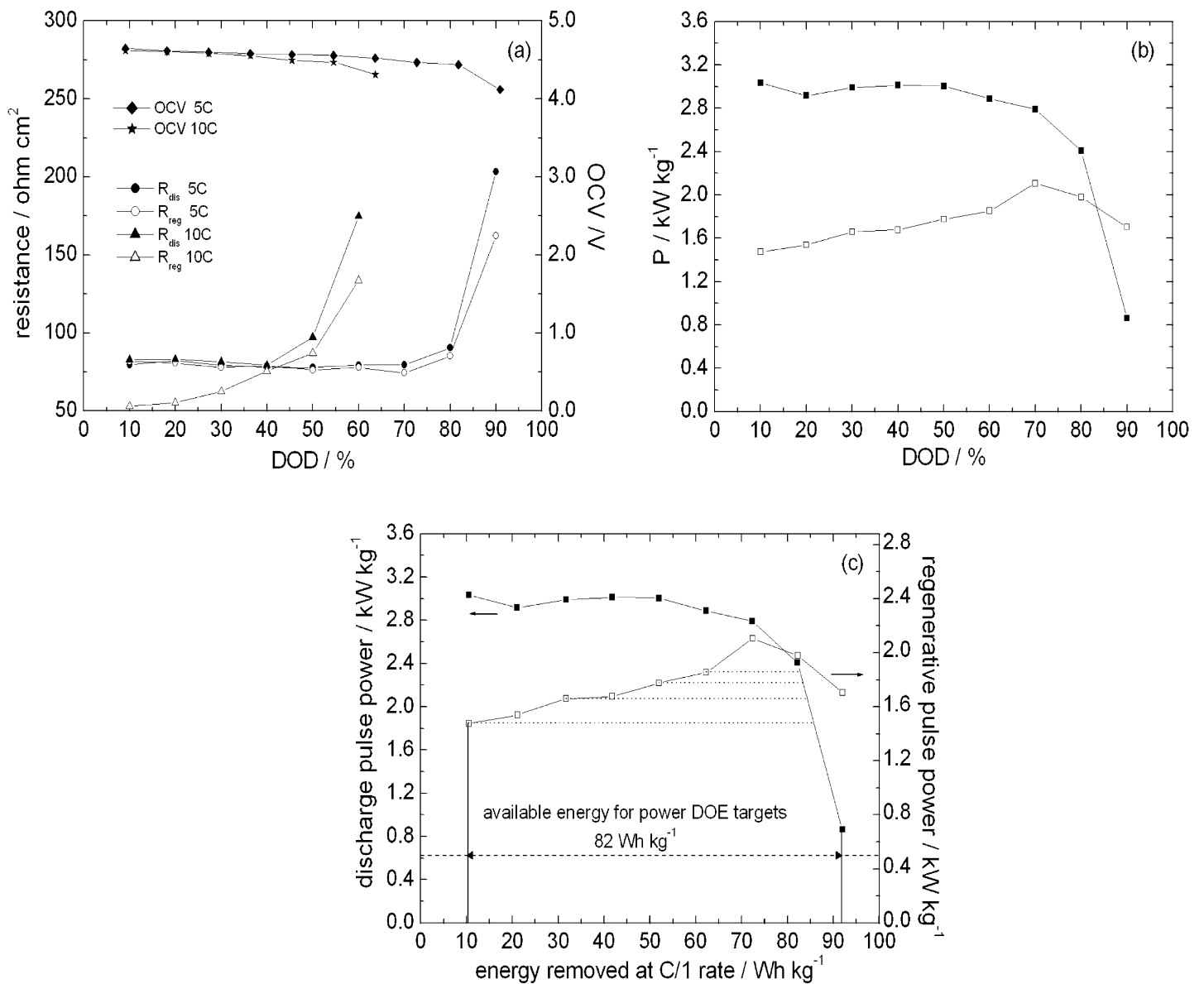
Figure 7. Cell with pVDF-NCC separator: (a) Open circuit voltage and resistance from discharge (full symbol) and regenerative (void symbol) pulses vs. DOD% from HPPC tests at 5C and 10C (the last ends at 60%DOD); (b) specific power of discharge (full symbol) and regenerative (void symbol) pulses from HPPC test at 5C vs. DOD%; (c) specific discharge power (full symbol) and regenerative (void symbol) from HPPC test at 5C with the two vertical axes rescaled in proportion of discharge and regenerative power goals vs energy removed during C/1 discharge of Fig.5a.
