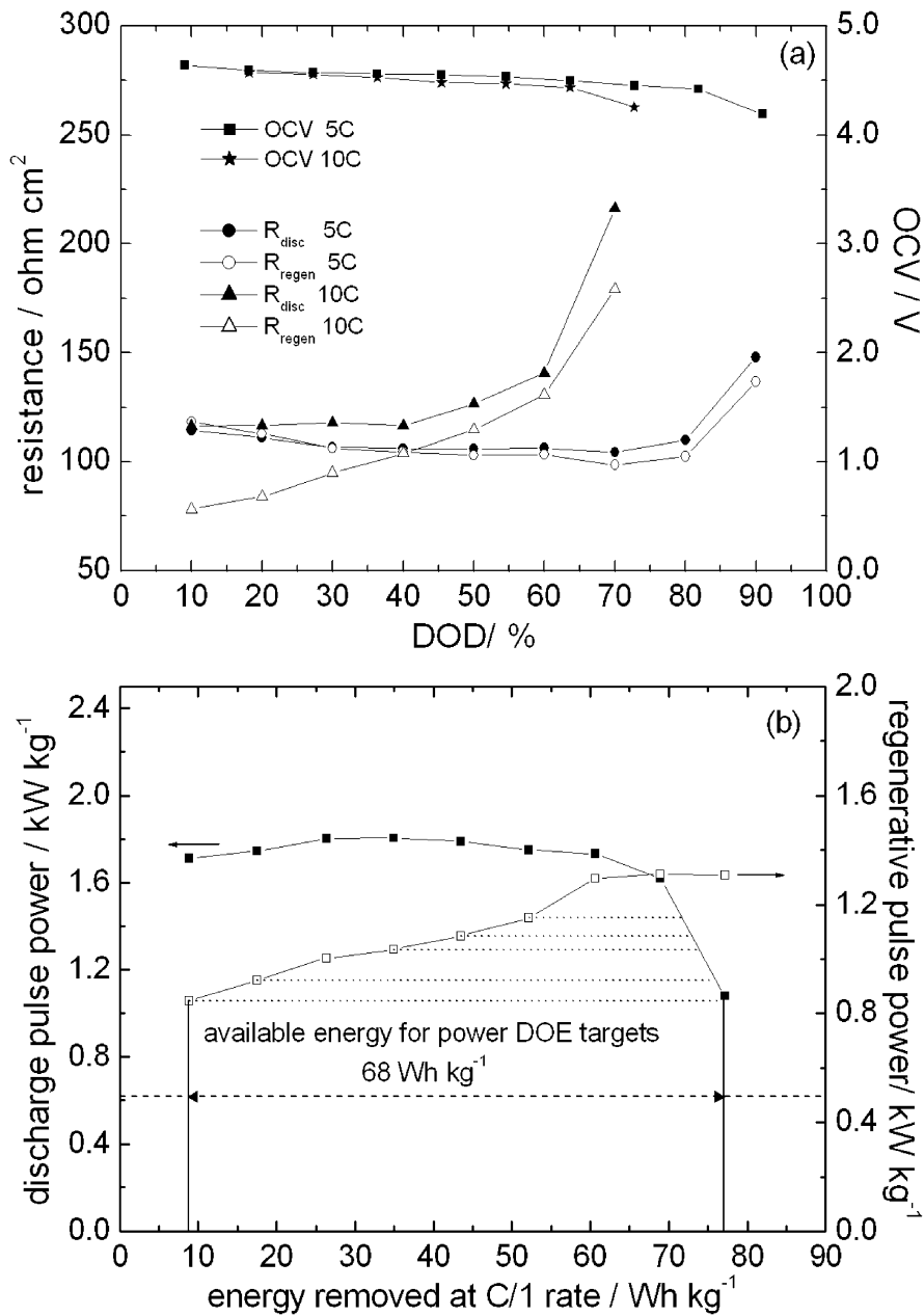
Figure 8. Cell with Celgard 2400 separator: (a) Open circuit voltage and resistance from discharge (full symbol) and regenerative (void symbol) pulses vs. DOD% from HPPC tests at 5C and 10C (the last ends at 70%DOD); (b) specific discharge power (full symbol) and regenerative (void symbol) from HPPC test at 5C with the two vertical axes rescaled in proportion of discharge and regenerative power goals vs energy removed during C/1 discharge of Fig.5b.
