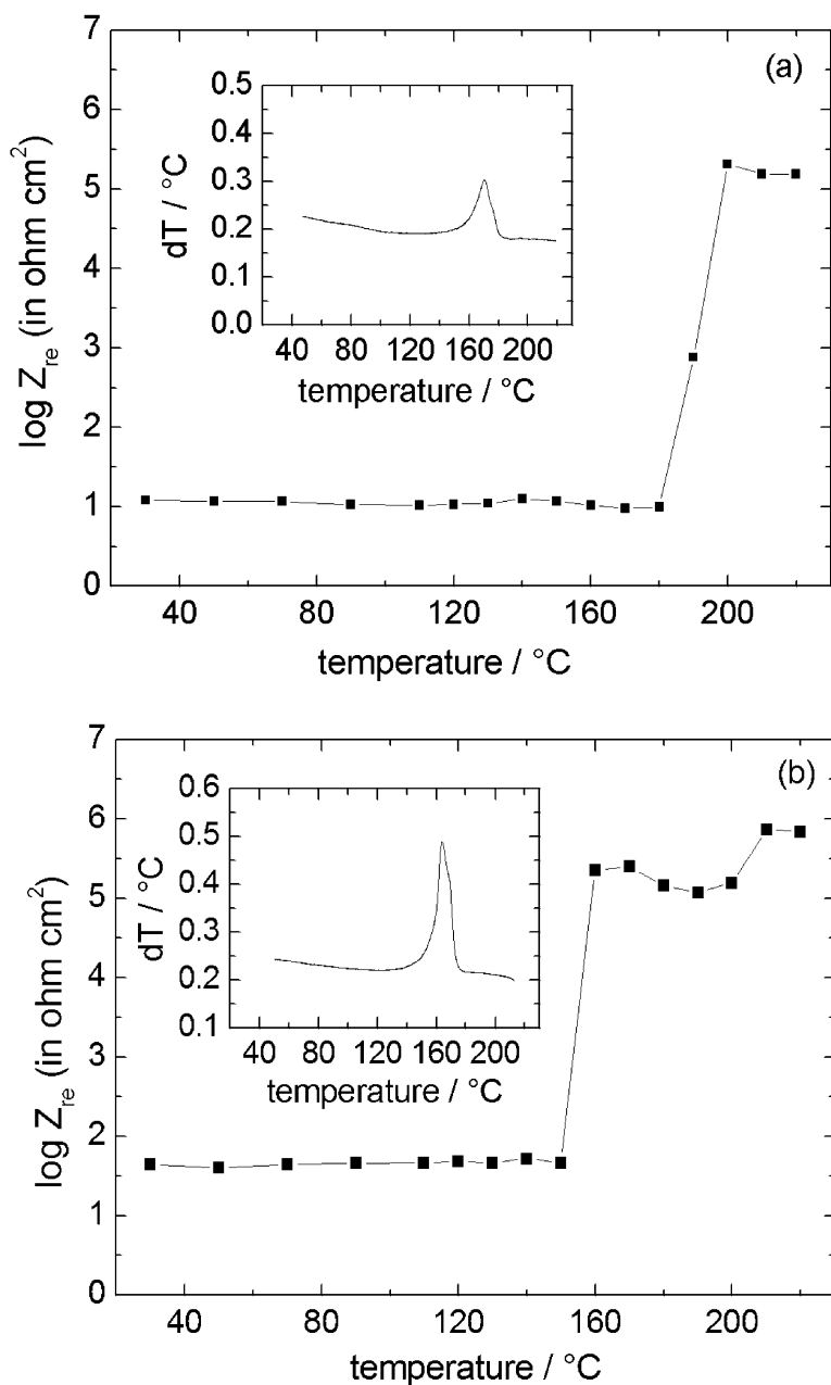
Figure 3. Logarithm Z_{re} , at 1 kHz vs. temperature over shutdown tests of electrolyte-soaked separators (a) pVDF-NCC and (b) Celgard 2400. Insets display the DTA traces ( 5^{\circ}\text{C min}^{-1} ) of dry separators.
