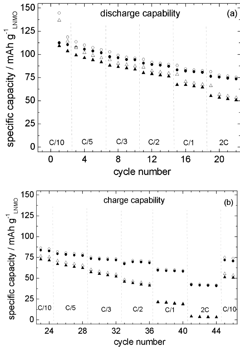
Figure 4. Comparison of discharge (a) and charge (b) capability of cells with pVDF-NCC (circle) and Celgard ® 2400 separator (triangles). Charge is indicated by void and discharges by full symbols.
