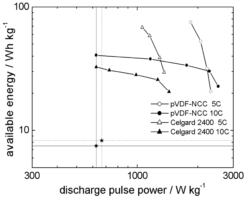
Figure 9. Plots of the available energy for a given pulse-power vs. discharge pulse power for cells with pVDF and Celgard ® 2400 separators from HPPC test at 5C and 10C.
