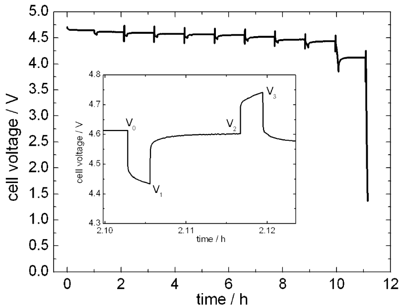
Figure 6. Cell voltage profile over HPPC at 5C of the cell with pVDF-NCC separator. In the inset, the magnification of the discharge and regenerative pulses at 10% DOD.
