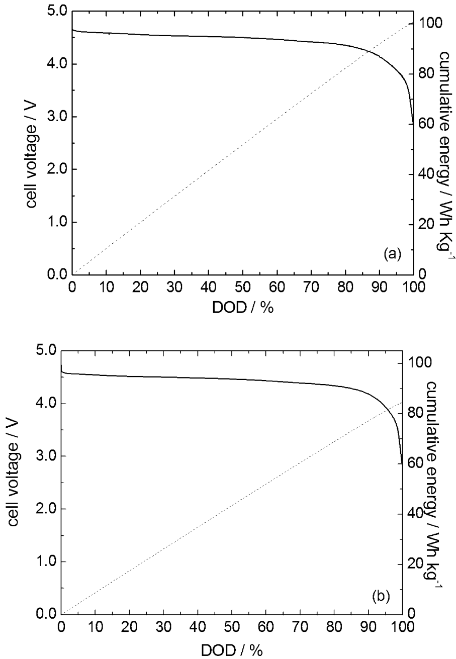
Figure 5. Discharge voltage profile (solid line) and delivered specific energy (dashed line) at C/1 effective rate vs. DOD of the cells with (a) pVDF-NCC and (b) Celgard ® 2400.
