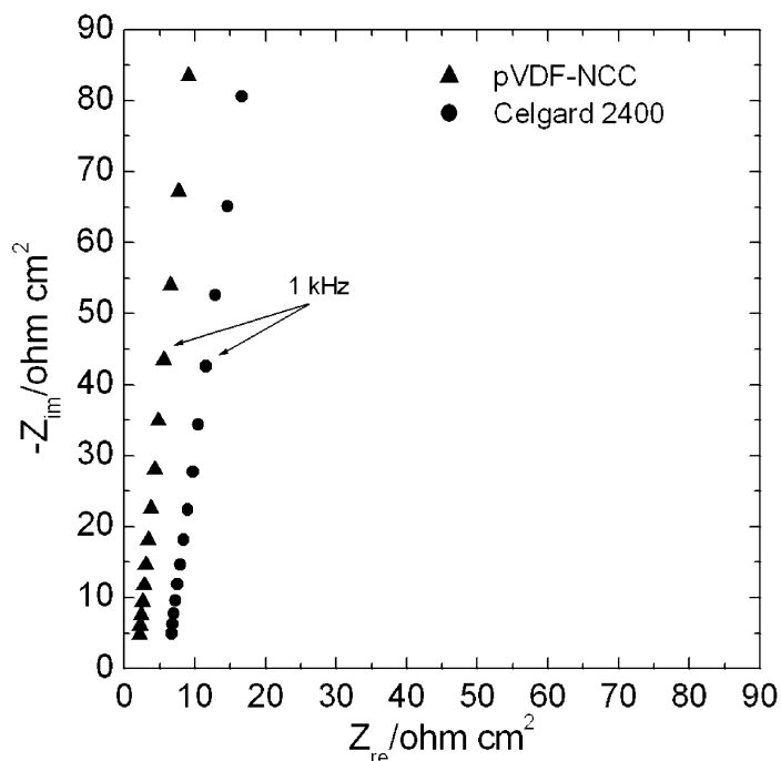
Figure 2. IS spectra of the electrolyte-soaked pVDF-NCC and Celgard ® 2400 separators at 30°C (10 kHz -0.501 kHz).
