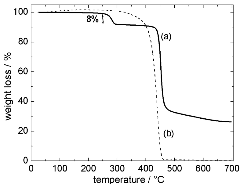
Figure 1. Thermogravimetric analysis of dry separators (a) pVDF-NCC and (b) Celgard ® 2400, in Ar flux (5 °C min -1 ).
