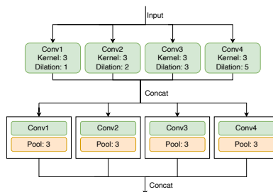
Figure 3. Dilated CNN block for frontend for 1D-input
