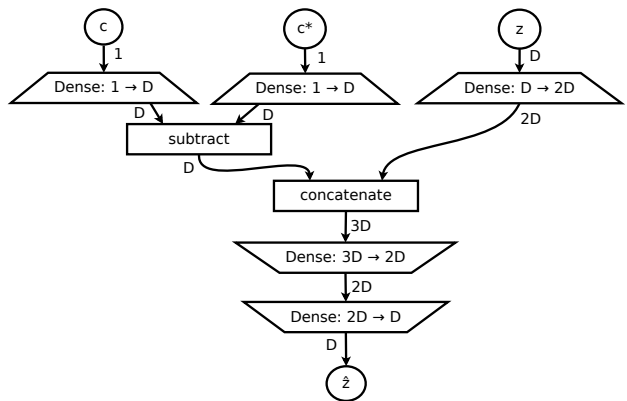
Figure 2. Implementation of SeNT-Gen neural traversal function \mathcal{T}_k(z, c_k, c_k^*) . Input is the latent code z , and the desired attribute change from c_k to c_k^* . Each Dense layer includes ReLU activation, except for the Tanh activation on the final layer. Output is the latent code \hat{z} which approximates the solution z^* .
