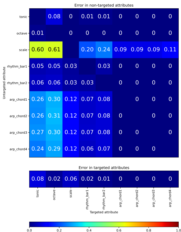
Figure 4. Accuracy of S2-VAE traversal, showing target deviation \Delta (bottom), and non-target deviation \nabla (top). Target attributes are on the horizontal axis, and non-targets on the vertical.
