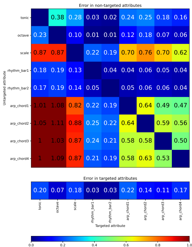
Figure 5. Accuracy of \beta -VAE traversal, showing target deviation \Delta (bottom), and non-target deviation \nabla (top). Target attributes are on the horizontal axis, and non-targets on the vertical.
