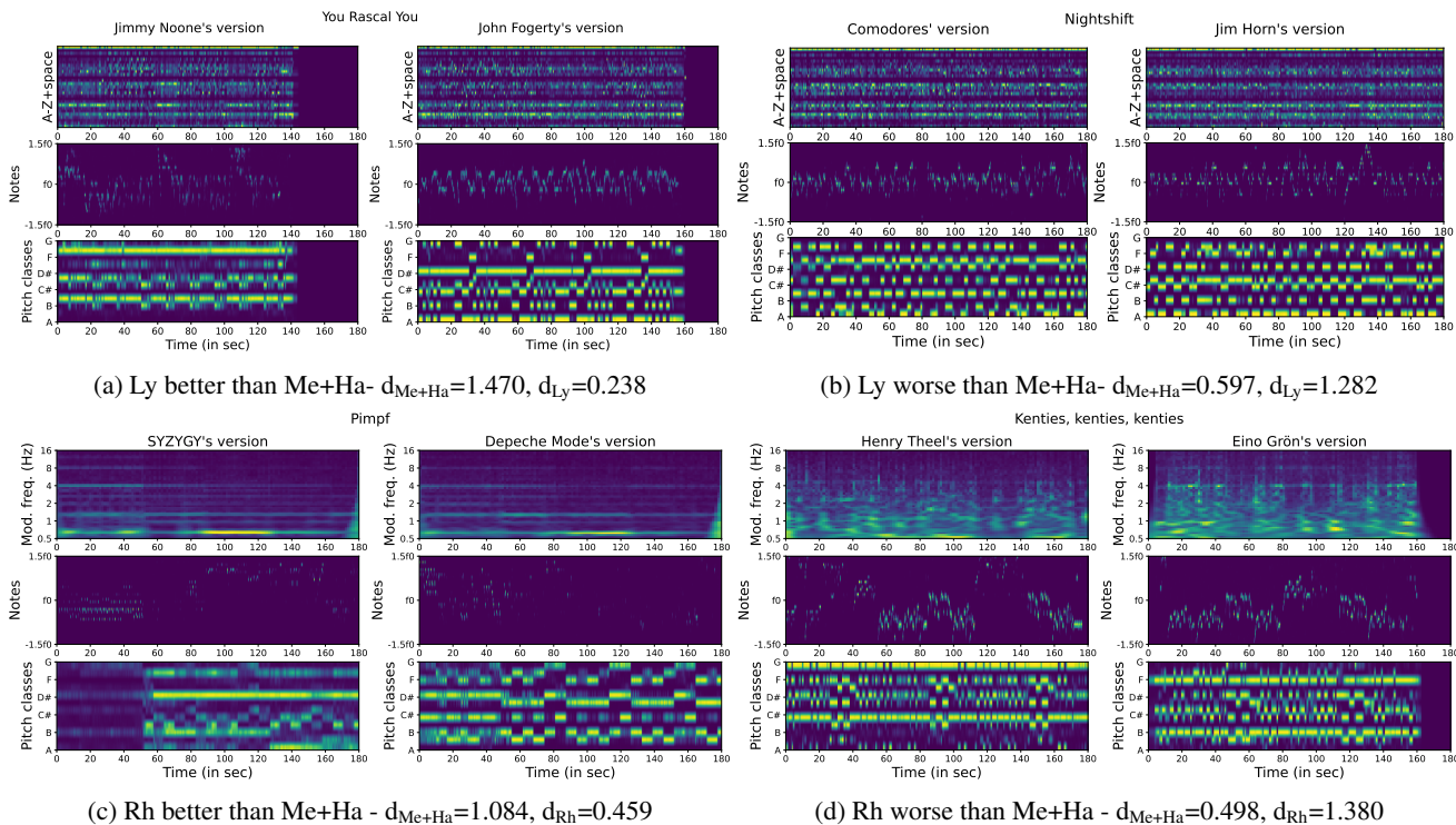
Figure 5: Examples for rhythm and lyrics : Rh > Me+Ha 5(c), Rh < Me+Ha 5(d), Ly > Me+Ha 5(a) and Ly < Me+Ha 5(b)
