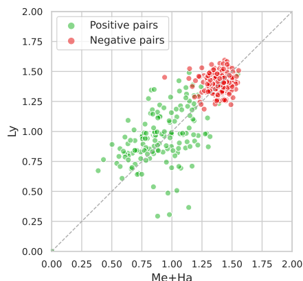
Figure 4: Pairwise distances for Me+Ha vs. Ly (500 pairs from SHS 4 ).
