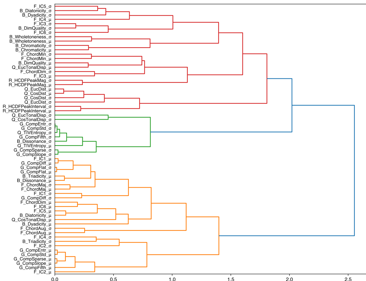
Figure 1. Hierarchical clustering of harmonic features computed at a 100ms resolution. The clustering is based on Spearman correlation distances using Ward’s linkage method.
