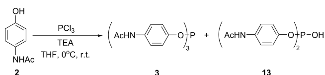
Scheme 2. Synthesis of Compound 3 from Paracetamol (2)
