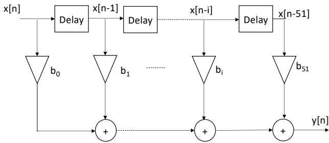
Fig. 4: FIR architecture
