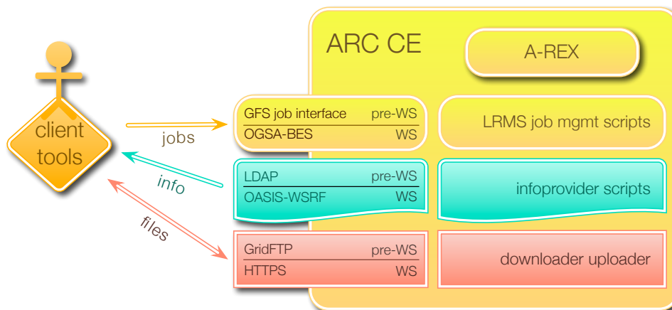
Figure 1.2: The interfaces and components of the ARC Computing Element
