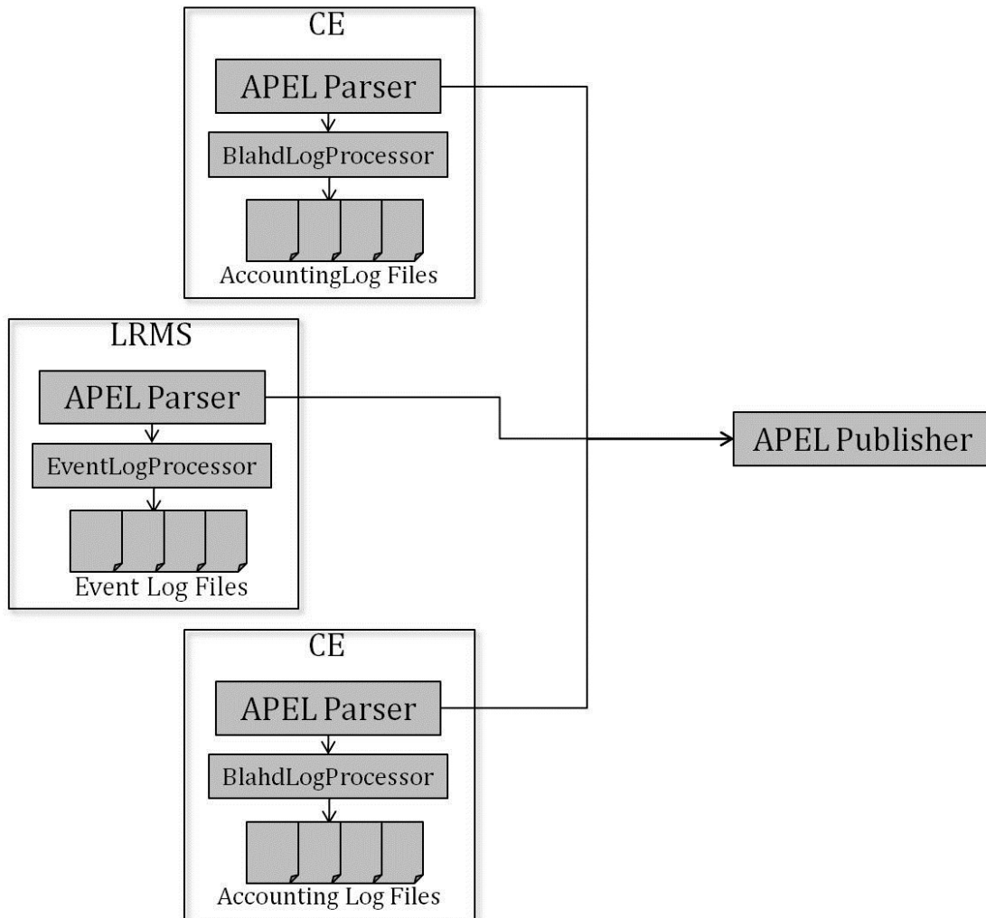
Figure 4: Multiple CEs
