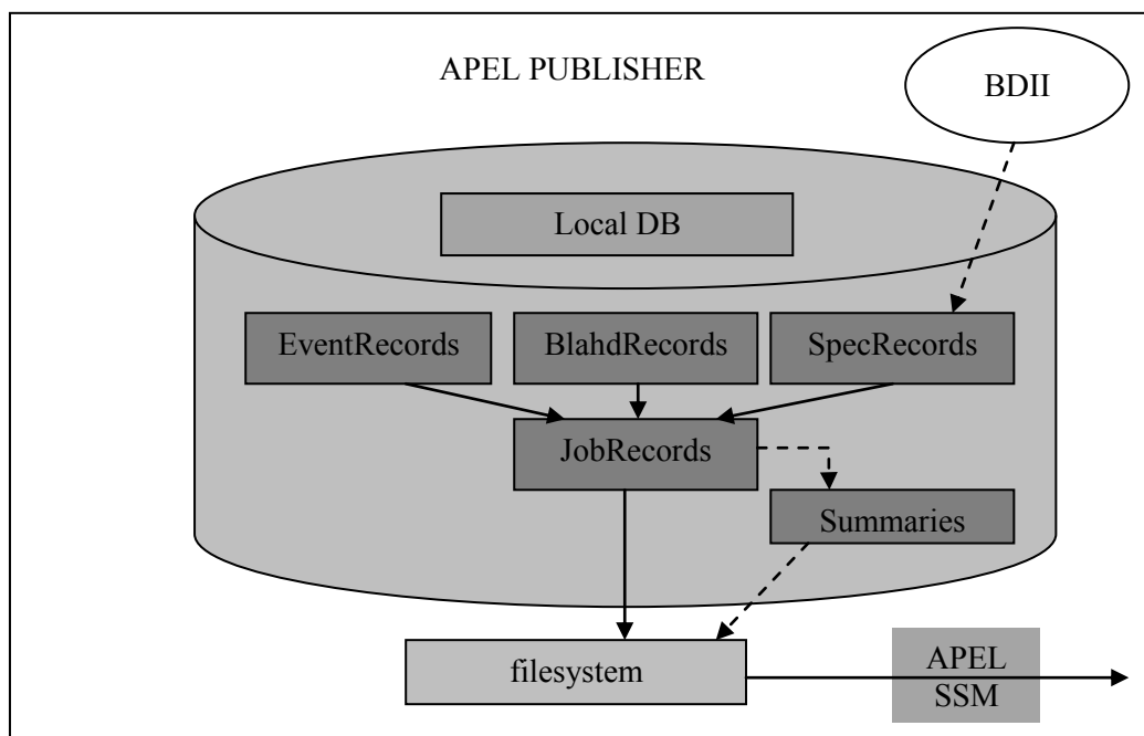
Figure 5: APEL Publisher
