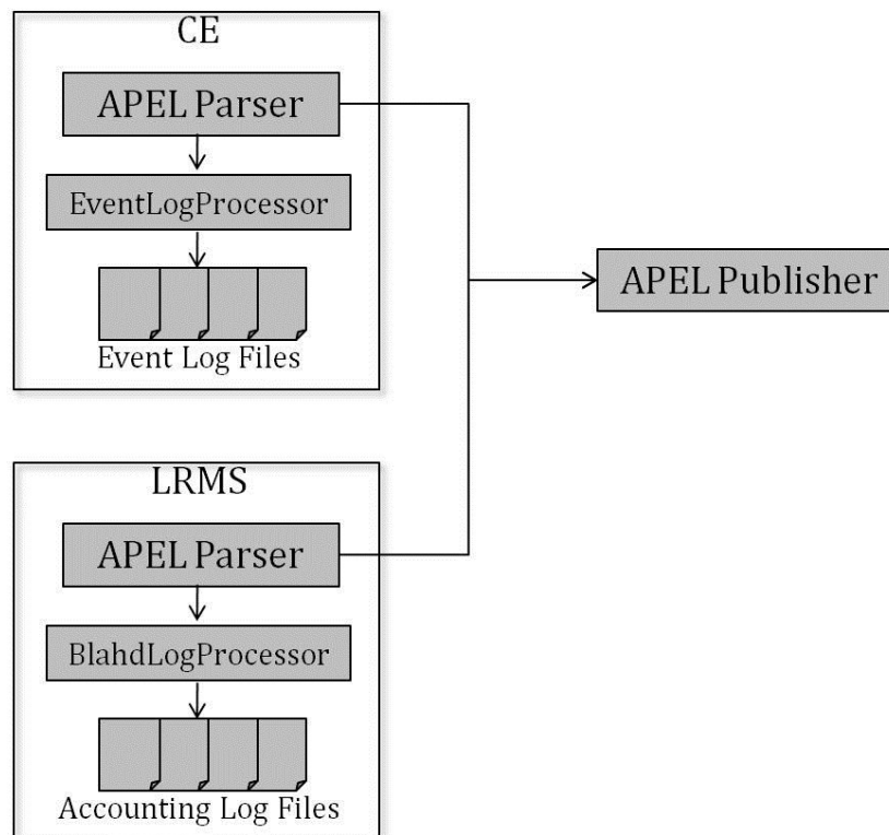
Figure 2: Separate LRMS/CE
