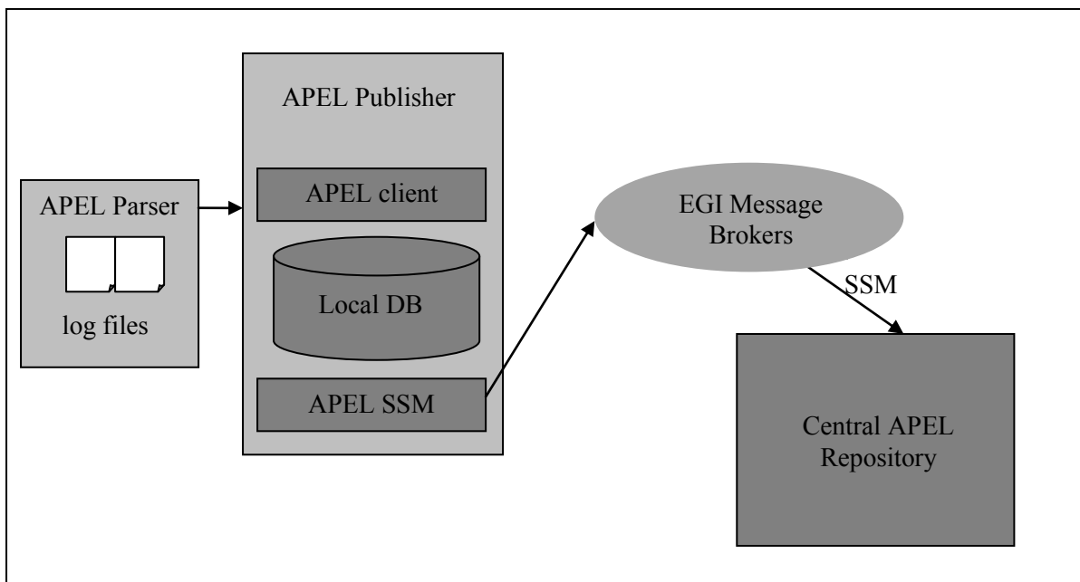
Figure 1: Overall Architecture
