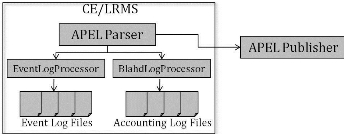
Figure 3: Combined LRMS/CE
