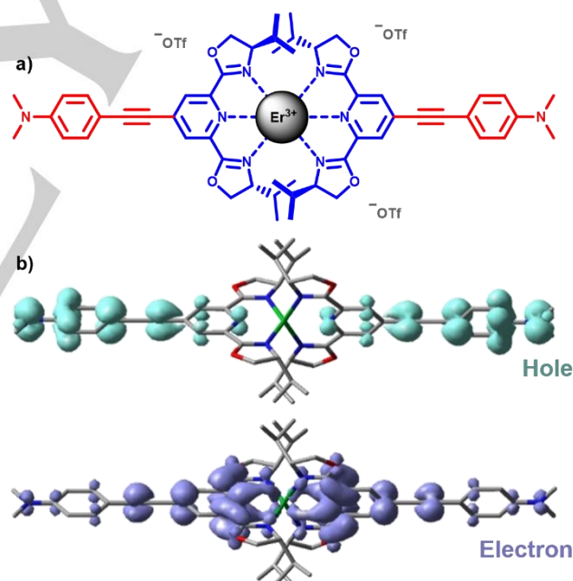
Figure 1. a) Structure of [Er(R,R)-L 2 ] 3+ ·3OTf - . b) Hole and electron distributions for the first excited state calculated for [Lu(R,R)-L 2 ] 3+ at CAM-B3LYP/def2-SVP/DZP[Lu]/B3LYP-D3BJ/def2-SVP/DZP[Lu] level; isovalue 0.0008.
