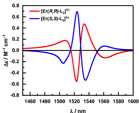
Figure 4. NIR-CD spectra of enantiomers of [\text{ErL}_2]\cdot 3\text{OTf} (4 mM). Spectra recorded in anhydrous \text{CDCl}_3 at room temperature.
