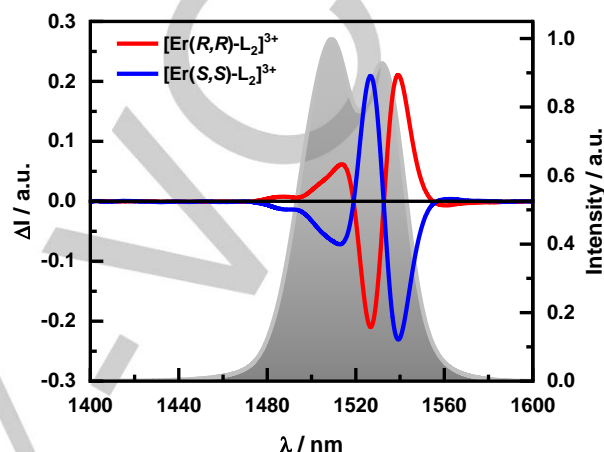
Figure 3. NIR-CPL spectra of enantiomers of [\text{ErL}_2]\cdot 3\text{OTf} (0.01 mM) with normalized average total emission traced in the background. Spectra recorded in anhydrous \text{CDCl}_3 at room temperature. \lambda_{ex} = 450 nm.
