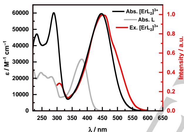
Figure 2. Absorption spectra of both the free ligand (grey) and complex (black), with the normalized complex excitation spectrum (red) superimposed ( \lambda_{em} = 1530 nm). All measurements were carried out in 0.01 mM anhydrous \text{CDCl}_3 solutions at room temperature.
