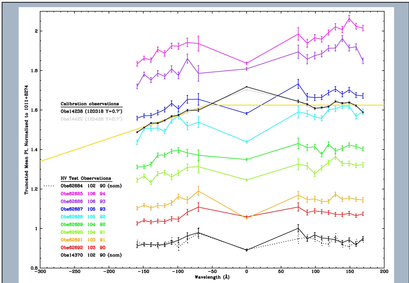
Fig. 1 - The mean pulse heights for 0th order and slices of dispersed HZ43 spectra, using the old gain calibration, and normalized to data obtained at the “old” voltage settings (ObsIDs 1011 and 8274). Colored curves and the bottom two black curves (solid and dotted) are for short test observations at various voltage settings. The different settings are denoted by a voltage “step” number for top and bottom plates listed after each ObsID. Settings for the blue curve (ObsID 62687) were chosen for the new operating voltage. The upper black and gray curves are for 10 ks calibration observations made with the new voltages. (0th order appears high for these two observations because they were made with Y-offset=0.7, which moves 0th order off a low-gain “burned-in” region at the on-axis aimpoint.) The gold line segments represent the gain correction factor used for pulse height-based background filtering in post-voltage-change observations.
