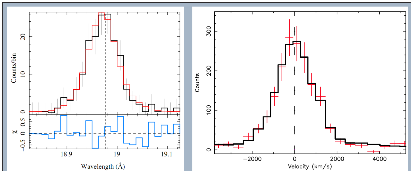
Fig. 2 - Velocity-broadened profiles of the H-like O VIII \lambda 18.97 \text{ Ly}\alpha line providing key diagnostics for O star winds. Left: The O VIII profile (black) seen in the LETG+ACIS-S spectrum of the O 9.5V “weak-wind” star \mu Col. A wind model with terminal velocity v_\infty = 1600 \text{ km s}^{-1} is shown in red, together with residuals in lower panel. The wind model indicates that nearly all the wind mass is at X-ray temperatures, eluding detection in the UV and alleviating the weak wind problem. From Huenemoerder et al. (2012). Right: The profile of the O VIII line in the LETG+HRC-S spectrum of the O9.5 supergiant \delta Ori that tests the collisionless shock scenario of Pollock (2007). Observations are illustrated in red, together with a fitted Gaussian model in black (note that the instrumental line spread function is also significant here). The rest wavelength is also shown. The HWHM of \sim 840 \text{ km s}^{-1} is possibly too small for a uniform, spherically-symmetric shocked-wind, and might betray the presence of self-obscuring clumps. From Raassen and Pollock (2013).
