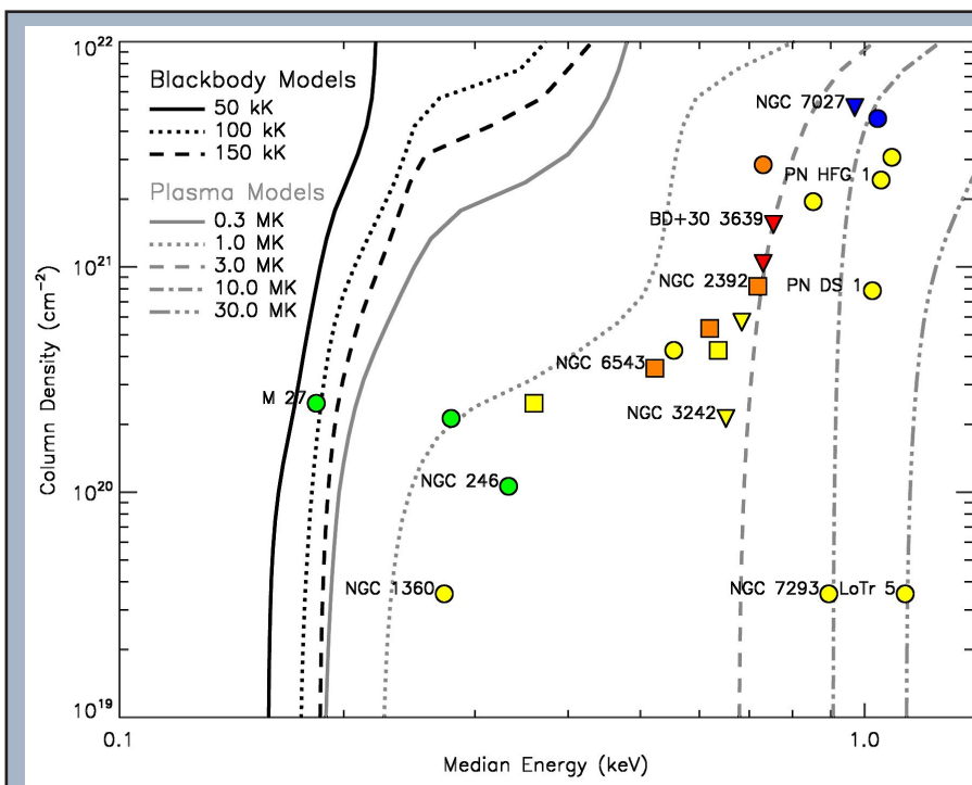
Fig. 5 - Plot of estimated intervening absorbing column density N_{\text{H}} vs. median source photon energy for CHANPLANS sample PNe detected as either diffuse or point-like X-ray sources (with symbols as in Fig. 3). The N_{\text{H}} estimates are obtained from measurements of the Balmer decrement (Frew 2008). We used a grid of spectral models (absorbed blackbody or absorbed thermal plasma) convolved with the Chandra -ACIS-S response to determine model median energies. Clearly, only the central star of the Dumbbell (M 27) can be modeled in terms of simple blackbody emission at temperatures expected of PN central stars; the rest of the central star X-ray sources appear to be affected (in some cases, dominated) by hotter, thermal plasma emission.
