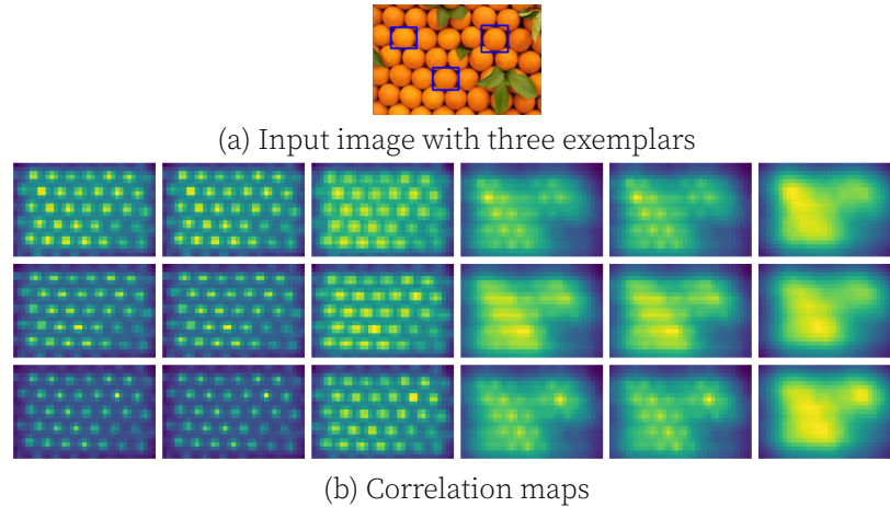
Figure 4. Figure shows an example of an input image (a) from FSC-147 with three exemplars (blue rectangles), and correlation maps between exemplar and image features (b), that are fed to the density prediction module. Each row corresponds to one exemplar, while each column corresponds to one combination of scale (3 scales) and feature output from third or fourth block of ResNet-18.
