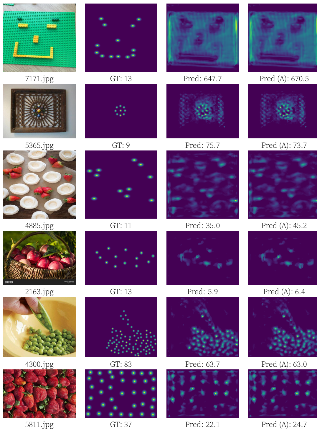
Figure 5. The first column represents input images, the second represents ground truth density maps, while the third and the fourth represent predicted density maps without and with test-time adaptation, respectively. The first three rows include cases where absolute error normalized by ground truth count is among the highest in the test set, while the last three rows where it is among the lowest.
