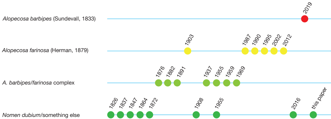
Fig. 1. — Schematic timeline of the different interpretations of Latreille's Lycosa accentuata Latreille, 1817. The names on the right are the most closely matching currently valid taxa, and the years refer to the major taxonomic publications detailed and discussed in Table 1. It is clear that the recent inversion of preceding usage, as proposed by Canard & Cruveillier (2019), contradicts all previous interpretations of the name. This figure should be read in conjunction with the detailed information in Table 1.
