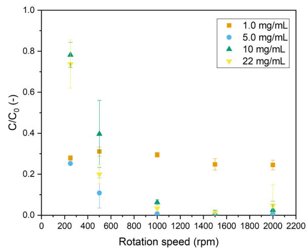
Figure 9. Normalized concentration of MB vs rotation speed for different catalyst concentrations/loadings [light input power 175 W (6.5 W/mL), \Phi_{\text{V,L}} = 13.5 mL/min, G/L ratio 1:1, 10 ppm MB].
