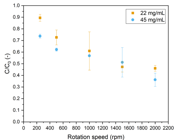
Figure 10. Normalized concentration of MB vs rotation speed for higher catalyst concentrations to test the limitations of the system [light input power 175 W (6.5 W/mL), \Phi_{\text{V,L}} = 27 mL/min, G/L ratio 1:1, 10 ppm MB].
