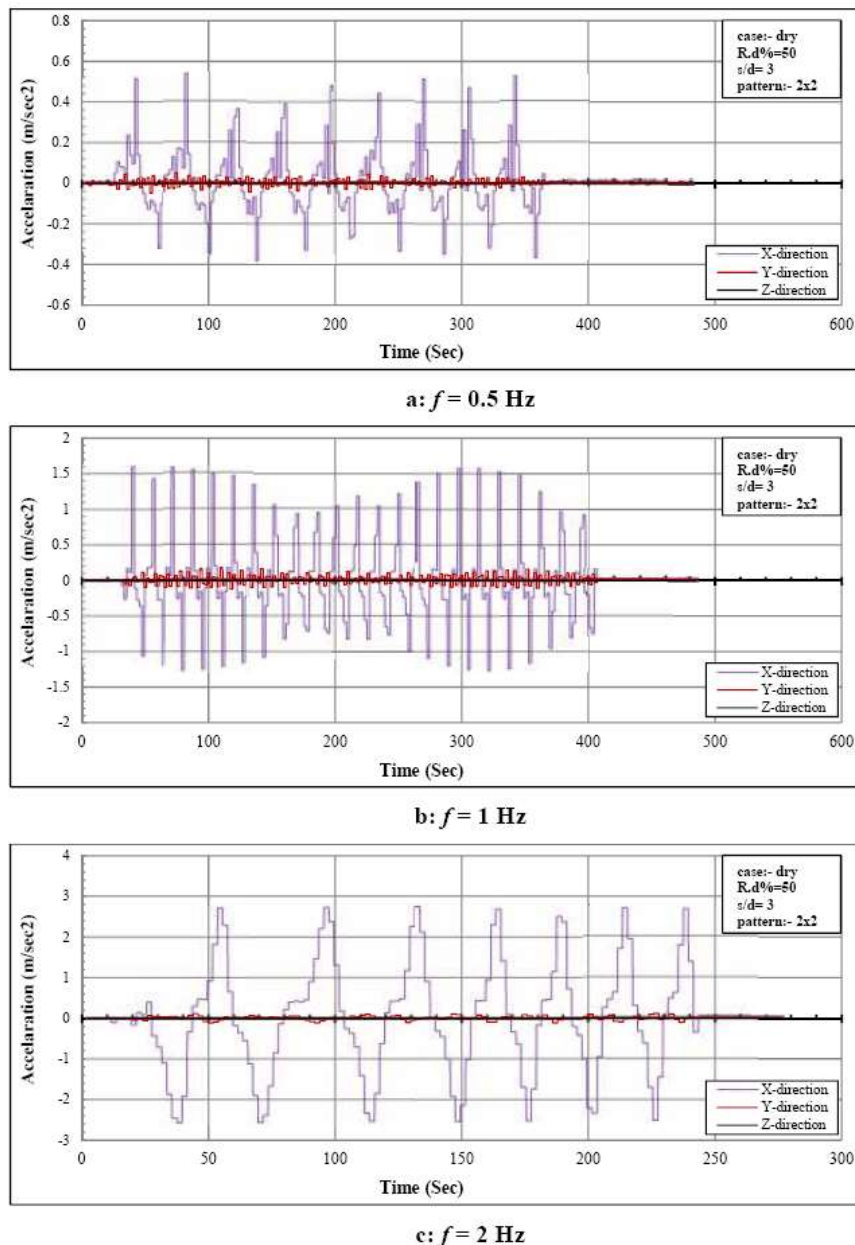
Figure 2: Acceleration time history in soil bed of pile group (2x2), in medium dry sand under different frequencies (a.0.5 Hz, b.1 Hz, c.2 Hz).
