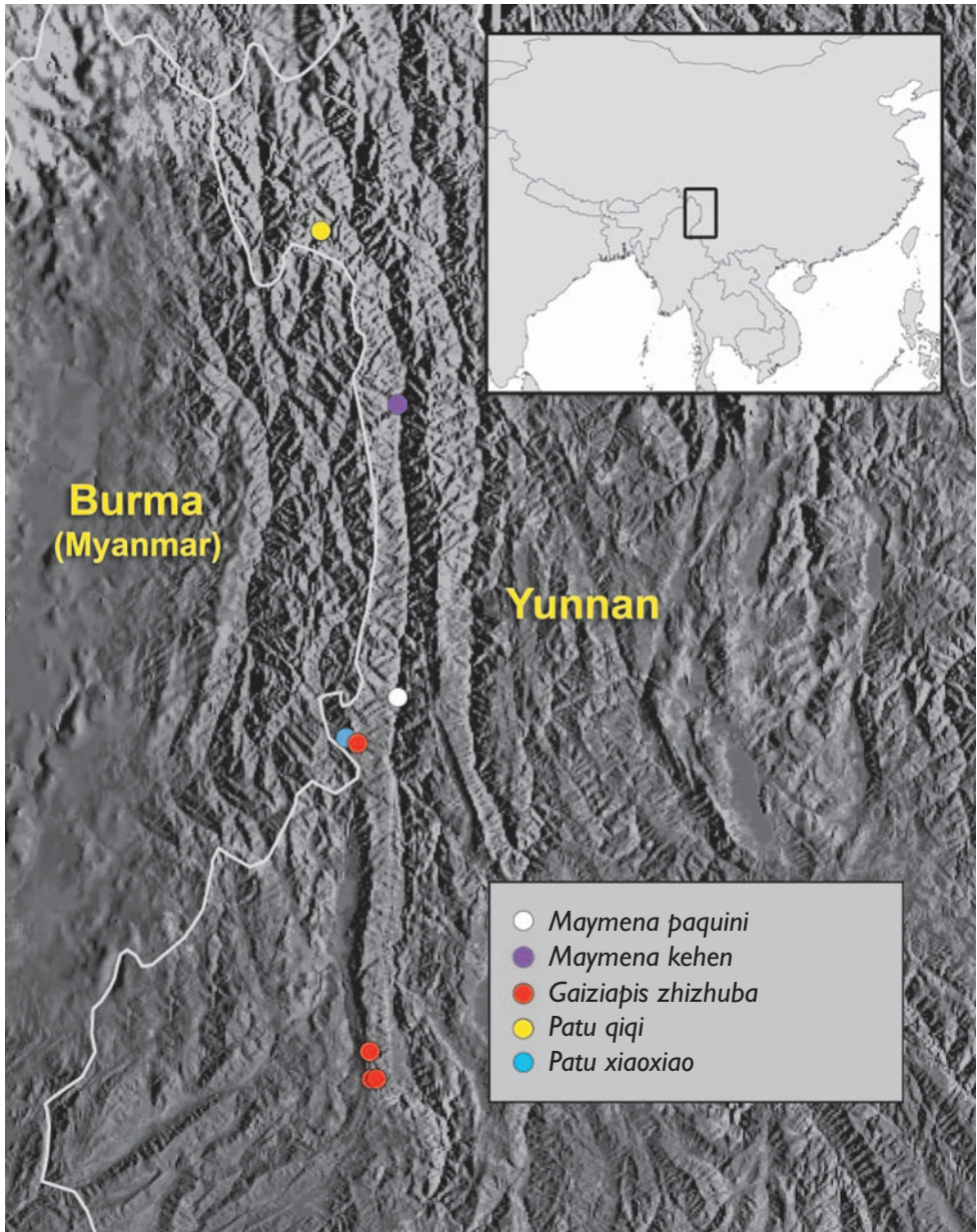
Figure 99. Distribution map, inset map shows study area. White: Maymena paquini sp. n.; purple: Maymena kehen sp. n.; red: Gaiziapis zhizhuba sp. n.; yellow: Patu qiqi sp. n.; blue: Patu xiaoxiao sp. n.
