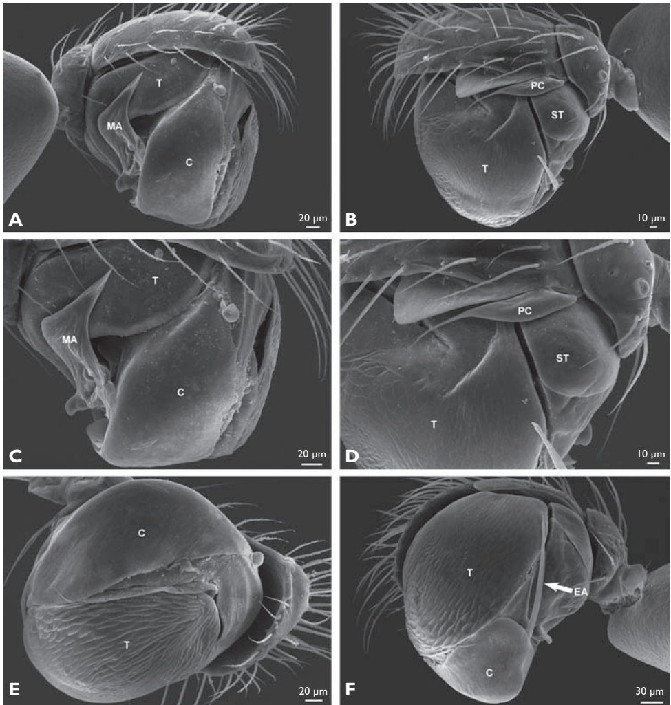
Figure 5. Ogulnius barbandrewsi sp. n. from Guocai He at Fucui, SEM of male palp. A, prolateral; B, retrolateral; C, prolateral, detail showing MA; D, retrolateral, detail showing paracymbium; E, apicoventral; F, retroventral showing EA. C: conductor; EA: embolic apophysis; MA: median apophysis; PC: paracymbium; ST: subtegulum; T, tegulum.
