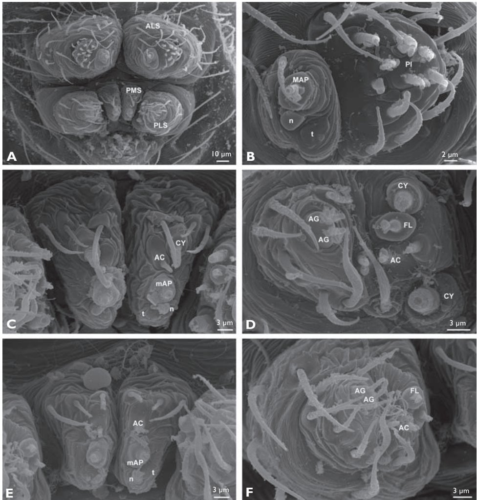
Figure 71. Patu jidanweishi sp. n. from Chang Yan He, SEM of spinnerets. A-D, female; E, F, male. A, spinnerets; B, ALS; C, E, PMS; D, F, PLS. AC: aciniform gland spigot; AG: aggregate gland spigot; ALS: anterior lateral spinneret; CY: cylindrical gland spigot; FL: flagelliform gland spigot; MAP: major ampullate gland spigot; mAP: minor ampullate gland spigot; n: nubbin; PI: piriform gland spigot; PLS: posterior lateral spinneret; PMS: posterior median spinneret; t: tartipore.
