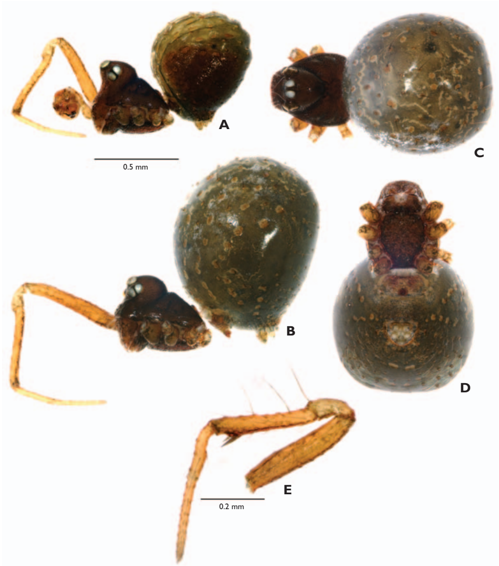
Figure 80. Crassignatha yinzhi from Xiao Hei Shan Nature Reserve. A, male, lateral; B, female, lateral; C, female, dorsal; D, female, ventral; E, male leg II, prolateral.
