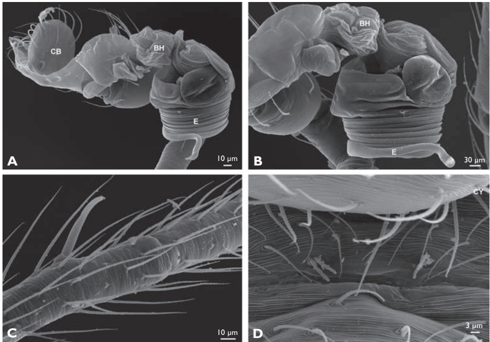
Figure 51. Chanea suukyii sp. n. from Maku ridge, SEM of male. A, B, palp, expanded, retrolateral; C, metatarsus I; D, epiandrous gland spigots. BH: basal hematodocha; CB: cymbium; E: embolus.
