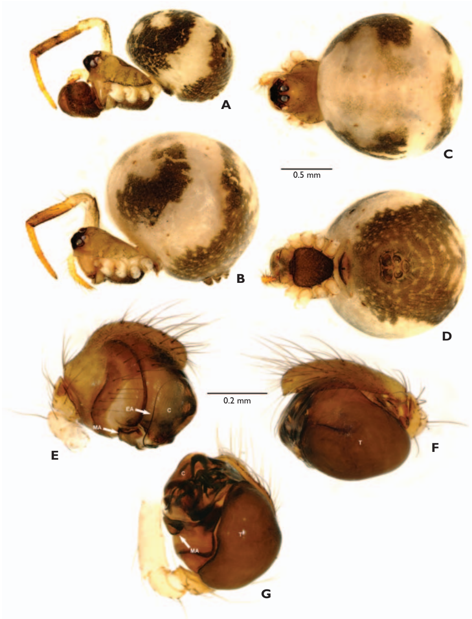
Figure 12. Wendilgarda muji sp. n. from Xiao Hei Shan Nature Reserve. A-D, habitus; E-G, male palp. A, male, lateral; B, female, lateral; C, female, dorsal; D, female, ventral; E, prolateral; F, retrolateral; G, ventral. C: conductor; EA: embolic apophysis; MA: median apophysis; T: tegulum.
