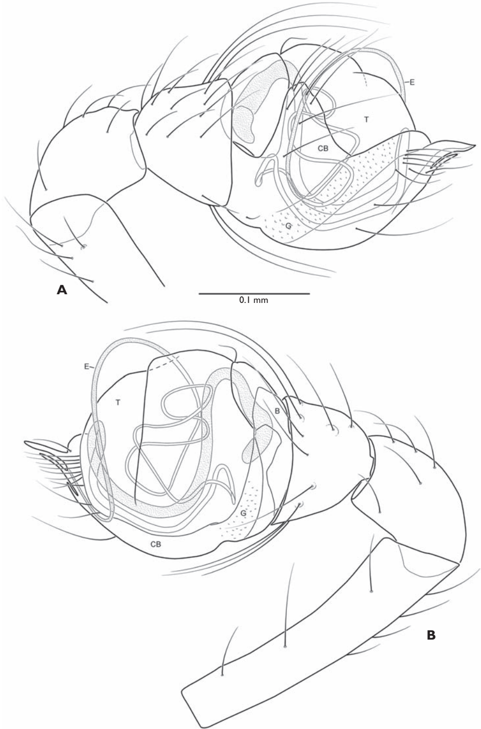
Figure 28. Mysmena goudao sp. n. from QiQi He, male palp. A, prolateral; B, retrolateral. B: base of cymbium; CB: cymbium; E: embolus; G: cymbial groove; T: tegulum.
