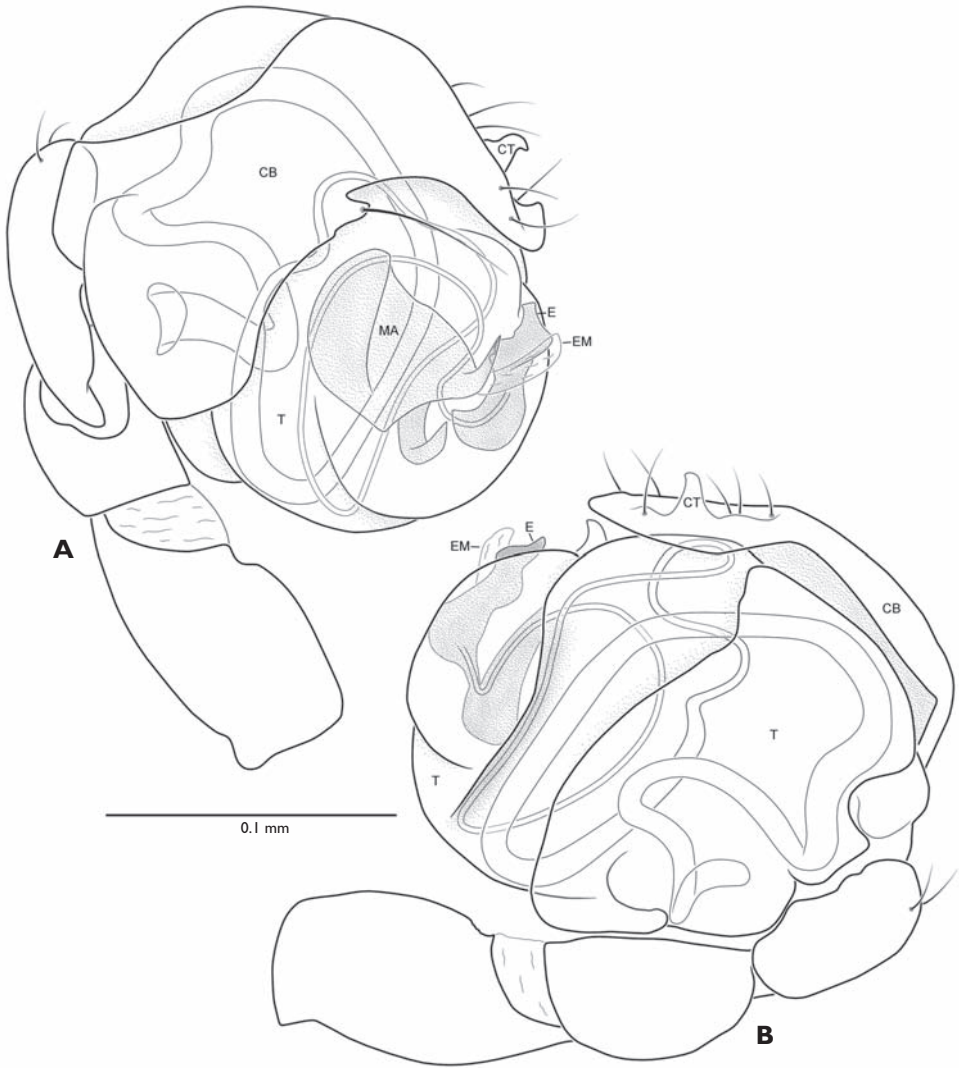
Figure 84. Crassignatha quanqu sp. n. from Bang Bie village, male palp. A, prolateral; B, retrolateral. CB: cymbium; CT: cymbial tooth; E: embolus; EM: embolic membrane; MA: median apophysis; T: tegulum.
