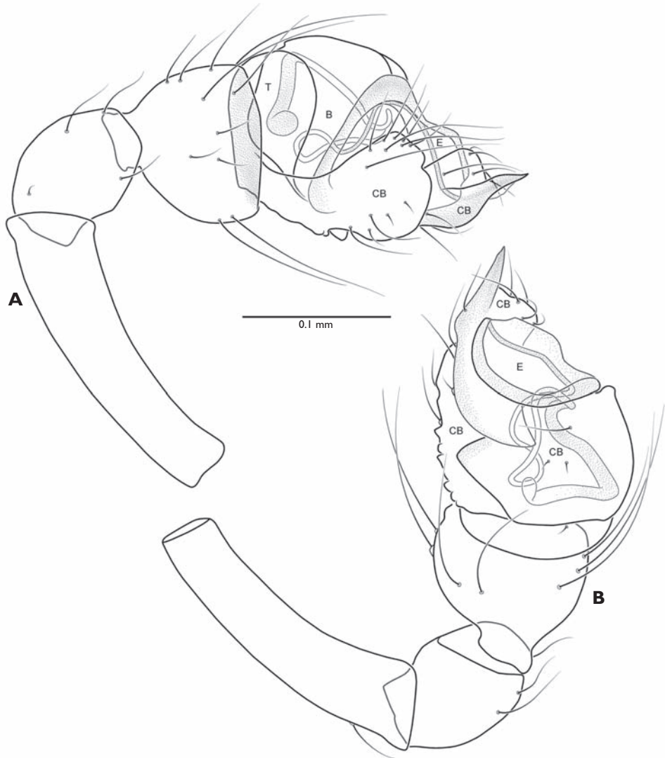
Figure 45. Gaoligonga zhusun sp. n. from Shilajia village, male palp. A, prolateral; B, retrolateral. B: base of cymbium; CB: cymbium; E: embolus; T: tegulum.
