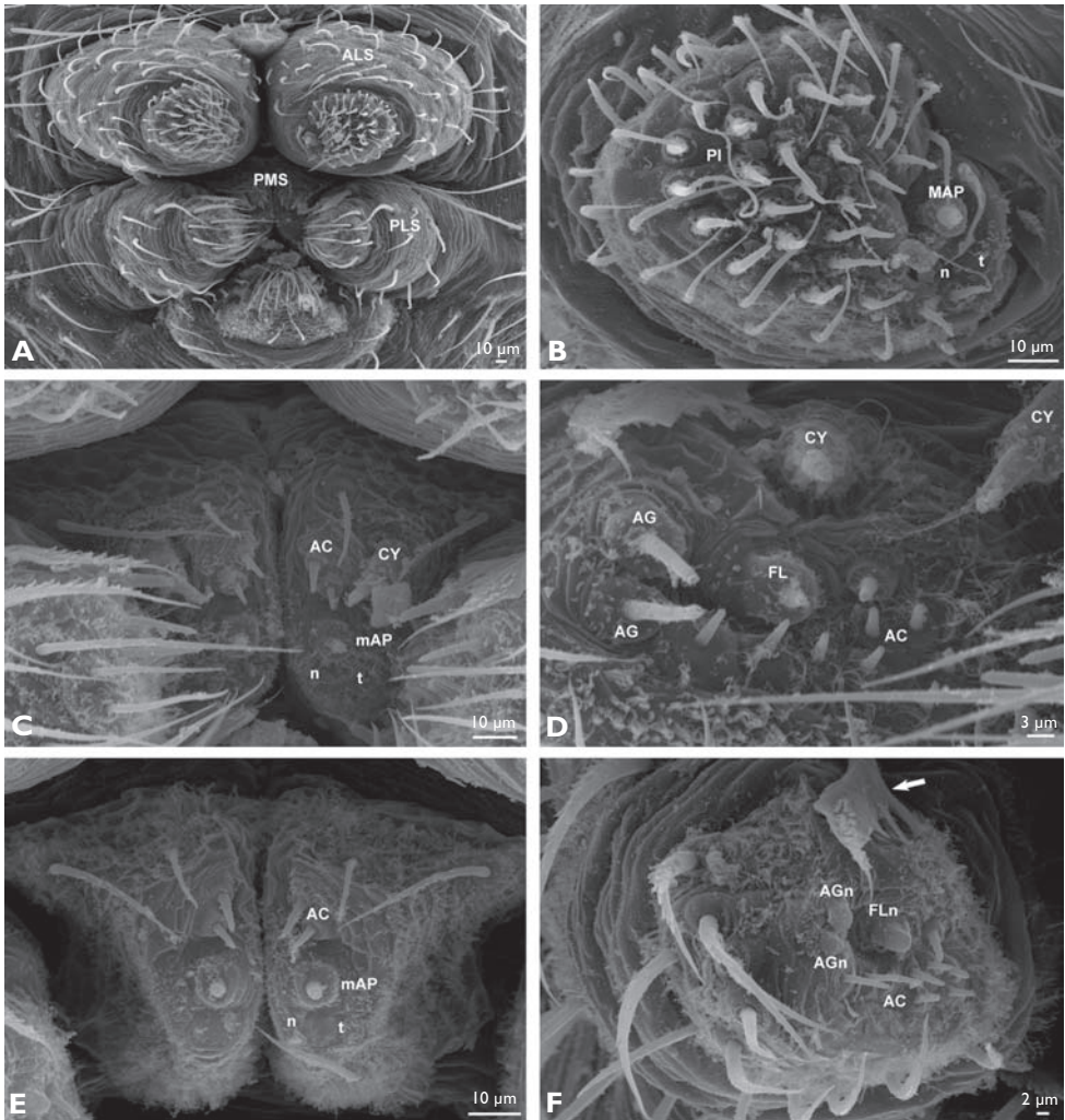
Figure 57. Maymena paquini sp. n. from Wayala Ku cave, SEM of spinnerets. A-D, female; E, F, male. A, spinnerets; B, PLS; C, E, PMS; D, F, PLS, arrow indicates modified PLS seta. AC: aciniform gland spigot; AG: aggregate gland spigot; AGn: aggregate gland spigot nubbin; ALS: anterior lateral spinneret; CY: cylindrical gland spigot; FL: flagelliform gland spigot; FLn: flagelliform gland spigot nubbin; MAP: major ampullate gland spigot; mAP: minor ampullate gland spigot; n: nubbin; PI: piriform gland spigot; PLS: posterior lateral spinneret; PMS: posterior median spinneret; t: tartipore.
