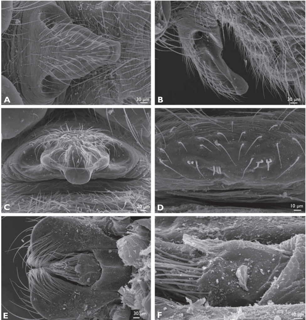
Figure 56. Maymena paquini sp. n. from Wayala Ku cave, SEM. A, epigynum, ventral; B, epigynum, lateral; C, epigynum, posterior; D, epiandrous gland spigots; E, female labrum, anterior, dorsal to the right; F, labrum, lateral, dorsal to the right.
