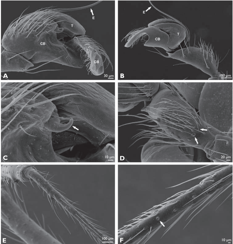
Figure 55. Maymena paquini sp. n. from Wayala Ku cave, SEM of male. A, palp, prolateral; B, palp, retrolateral; C, palp, prolateral detail, arrow indicates hook-like cymbial apophysis; D, palpal tibia, dorsal, arrows indicate trichobothria; E, metatarsus I; F, tarsus, arrow indicates tarsal organ. CB: cymbium; E: embolus; T: tegulum.
