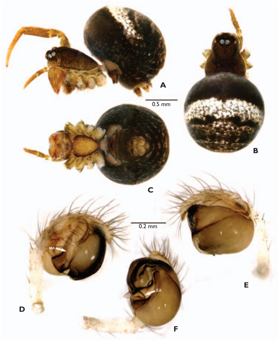
Figure 10. Zoma dibaiyin sp. n. from Pee He. A-C, female habitus; D-F, male palp. A, lateral; B, dorsal; C, ventral; D, prolateral; E, retrolateral; F, ventral. C: conductor; EA: embolic apophysis; MA: median apophysis; T, tegulum.
