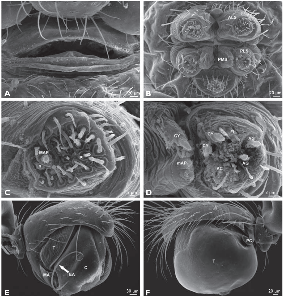
Figure 13. A-D, Zoma dibauiyin sp. n. from Pee He, SEM of female; E, F, Wendilgarda muji sp. n. from Xiao Hei Shan Nature Reserve, SEM of male palp. A, epigynum; B, spinnerets; C, ALS; D, PMS and PLS; E, prolateral; F, retrolateral. AC: aciniform gland spigot; AG: aggregate gland spigot; C: conductor; CY: cylindrical gland spigot; EA: embolic apophysis; FL: flagelliform gland spigot; MA: median apophysis; MAP: major ampullate gland spigot; mAP: minor ampullate gland spigot; n: nubbin; PC: paracymbium; PI: piriform gland spigot; T: tegulum.
