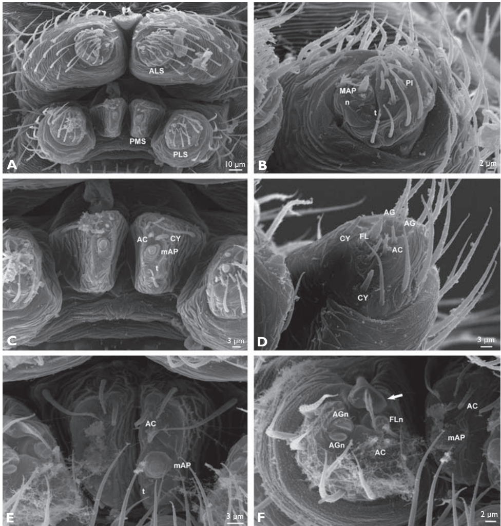
Figure 42. Gaoligonga changya sp. n., SEM. A-D, female; E, F, male. A, spinnerets; B, ALS; C, E, PMS; D, F, PLS, arrow indicates modified PLS seta. AC: aciniform gland spigot; AG: aggregate gland spigot; AGn: aggregate gland spigot nubbin; ALS: anterior lateral spinneret; CY: cylindrical gland spigot; FL: flagelliform gland spigot; FLn: flagelliform gland spigot nubbin; MAP: major ampullate gland spigot; mAP: minor ampullate gland spigot; n: nubbin; PI: piriform gland spigot; PLS: posterior lateral spinneret; PMS: posterior median spinneret; t: tartipore.
