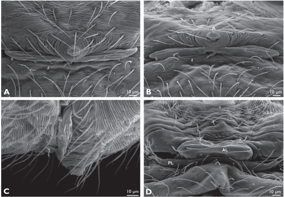
Figure 30. SEM, epigynum. A-C, Mysmena shibali sp. n. from Shibali; D, Simaoa yaojia sp. n. from Yaojiaping. A, D, ventral view; B, posterioventral view; C, lateral view. AL: anterior lobe; PL: posterior lobe.
