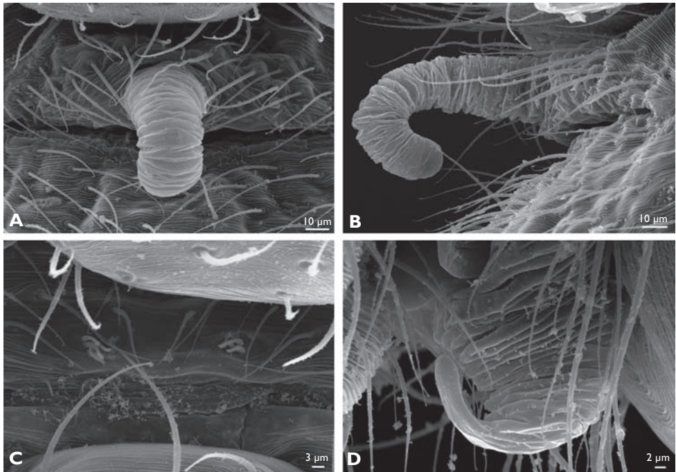
Figure 18. A-C, Mysmena changouzi sp. n. from No. 12 Bridge Camp area, SEM; D, Mysmena jinlong sp. n. from Danzhu He drainage, SEM of female. A, epigynum, ventral; B, epigynum, lateral, dorsal to the right; C, male epiandrous gland spigots; D, epigynum, lateral.
