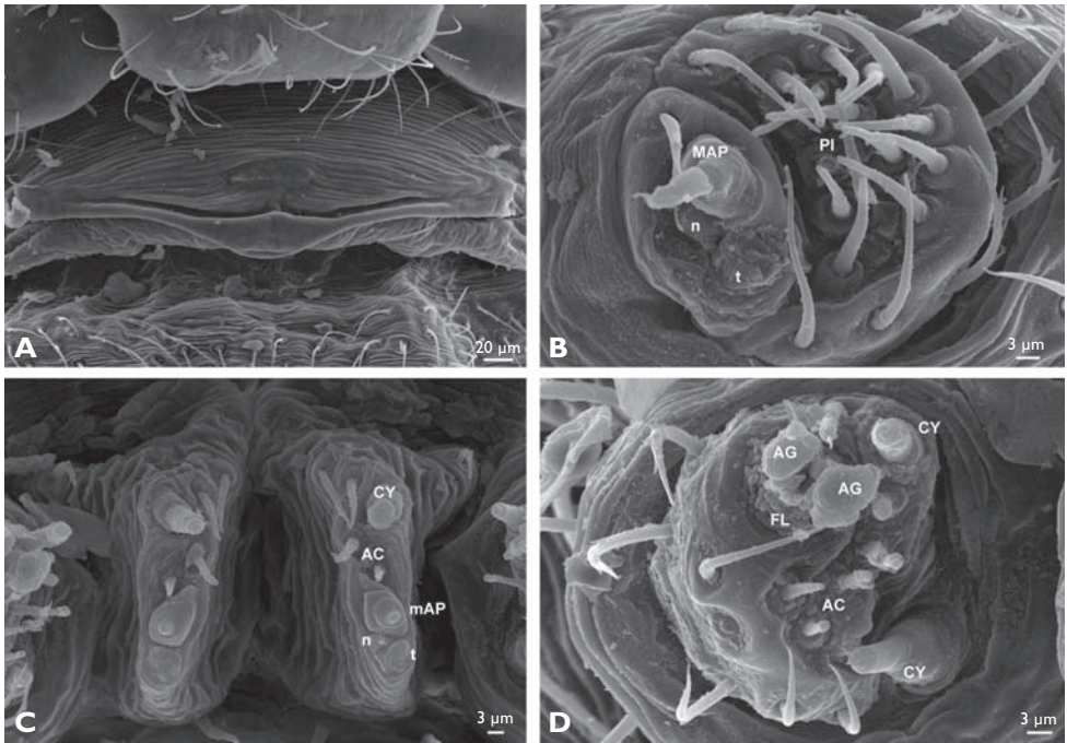
Figure 6. Ogulnius barbandrewsi sp. n. from Guocai He at Fucui, SEM of female. A, epigynum; B, ALS; C, PMS; D, PLS. AC: aciniform gland spigot; AG: aggregate gland spigot; CY: cylindrical gland spigot; FL: flagelliform gland spigot; MAP: major ampullate gland spigot; mAP: minor ampullate gland spigot; n: nubbin; PI: piriform gland spigot, t: tartipore.
