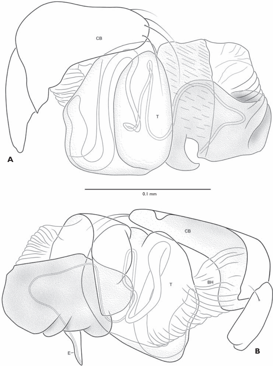
Figure 73. Patu qiqi sp. n. from QiQi He, slightly expanded male palp. A, prolateral; B, retrolateral. BH: basal hematodocha; CB: cymbium; E: embolus; T: tegulum.
