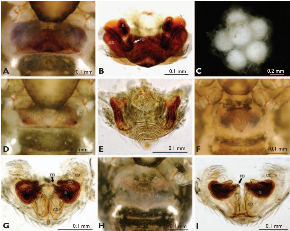
Figure 43. A-C, Gaoligonga changya sp. n. from QiQi He; D, E, Gaoligonga zhusun sp. n. from Shilajia village; F-G, Mosu nujiang sp. n. from Pee He; H, I, Mosu huogou sp. n. from Haban Falls. A, D, F, H, epigynum, ventral view; B, E, G, I, cleared vulva, dorsal view; C, eggs. CD: copulatory duct; FD: fertilization duct; S, spermatheca.
