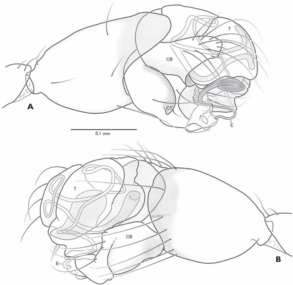
Figure 36. Simaoa kavanaugh sp. n. from Xiao Hei Shan Nature Reserve, male palp. A, prolateral; B, retrolateral. CB: cymbium; CT: cymbial tooth; E: embolus; T: tegulum.
