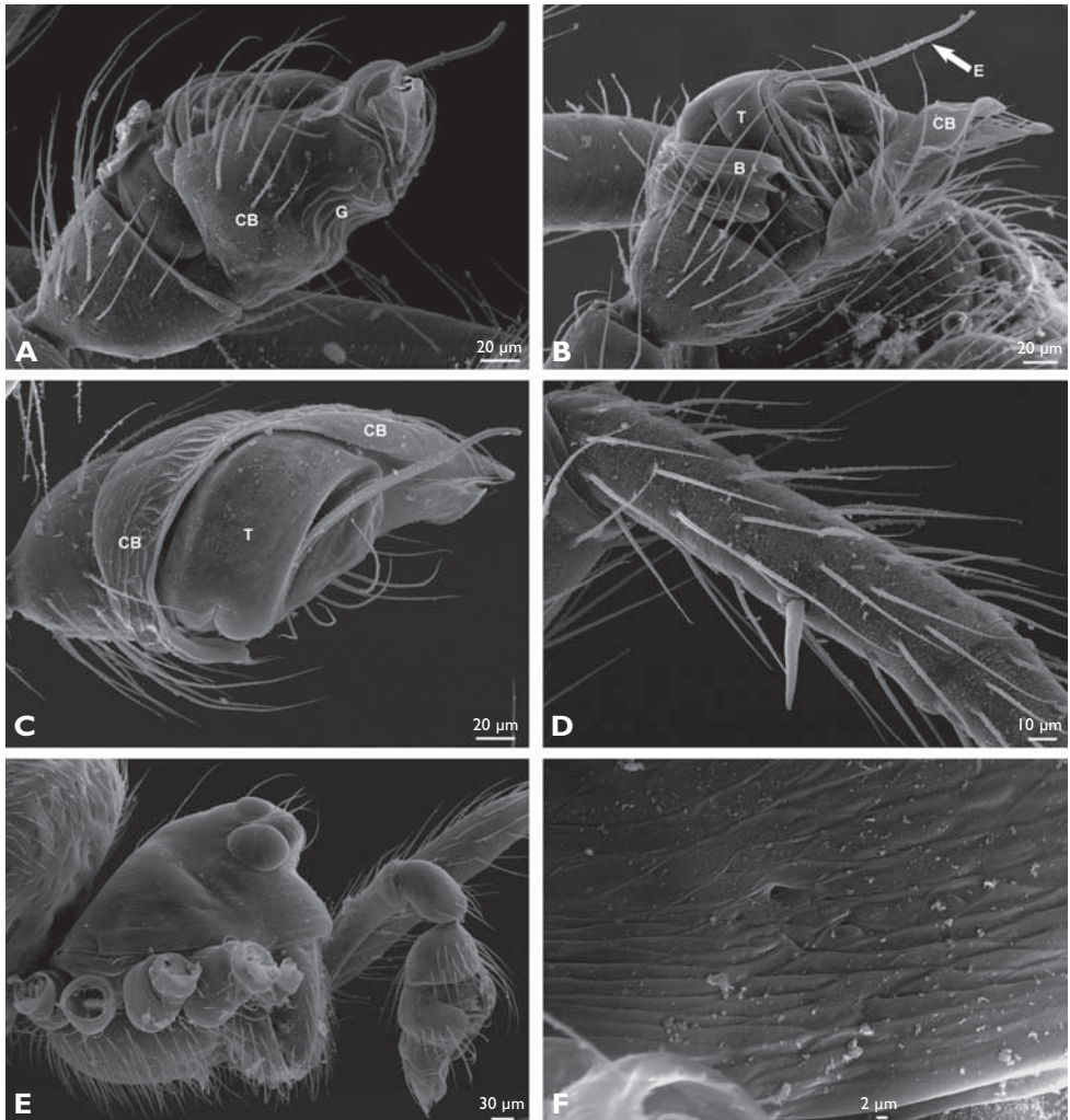
Figure 17. Mysmena changouzi sp. n. from No. 12 Bridge Camp area, SEM of male. A, male palp, prolateral; B, male palp, retrolateral; C, male palp, ventral; D, metatarsus I; E, prosoma, lateral; F, detail, carapace showing lateral pore. B: base of cymbium; CB: cymbium; E: embolus; G: cymbial groove; T: regulum.
