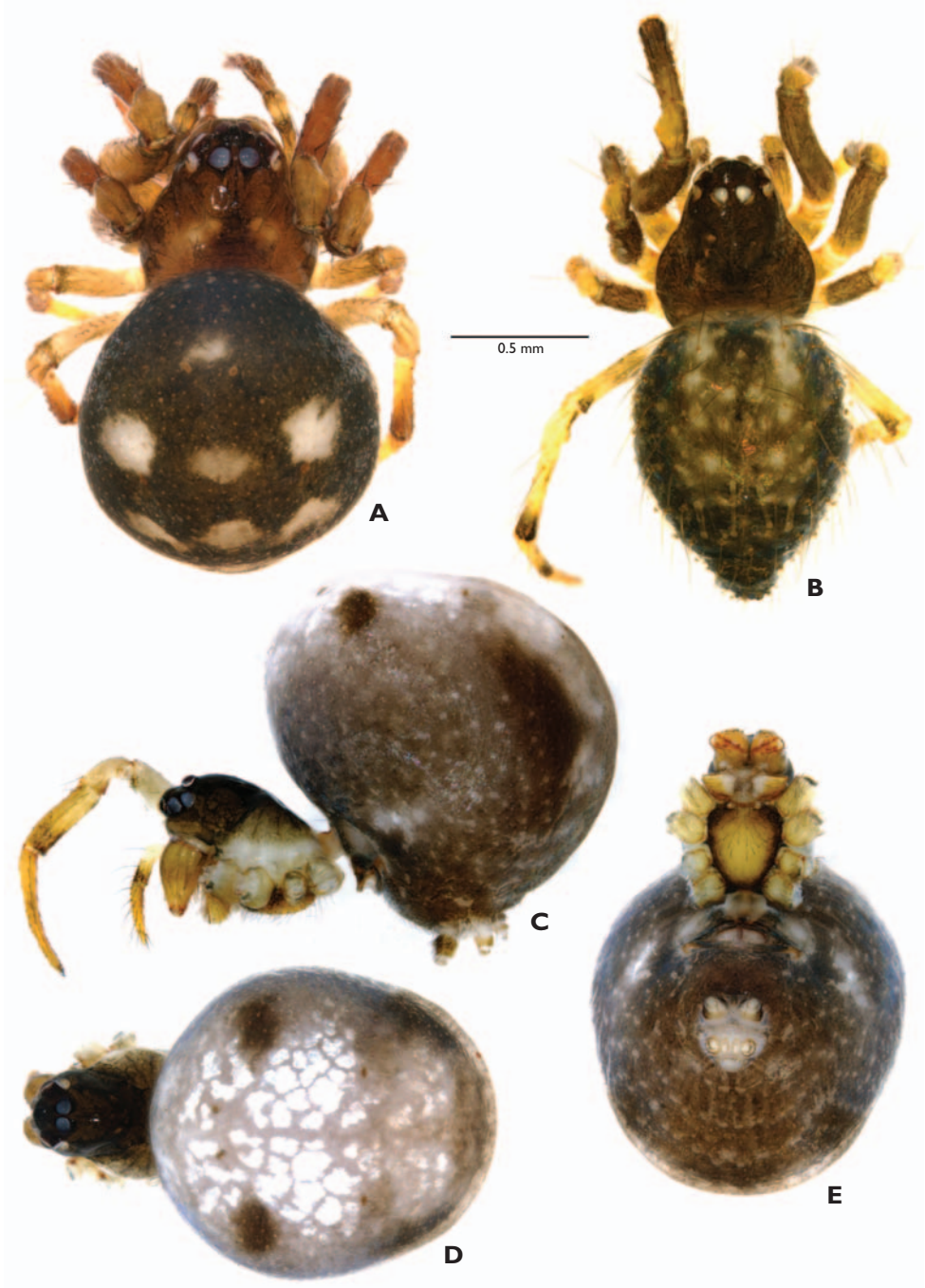
Figure 8. A, Baalzebub nemesis sp. n. from No. 12 Bridge Camp area; B, Coddingtonia euryopoides sp. n. from Zaochang He at Baihualing village; C-E, Theridiosoma diwang sp. n. from Xiao Hei Shan Nature Reserve, female. A, B, D, female, dorsal; C, female, lateral; E, female, ventral.
