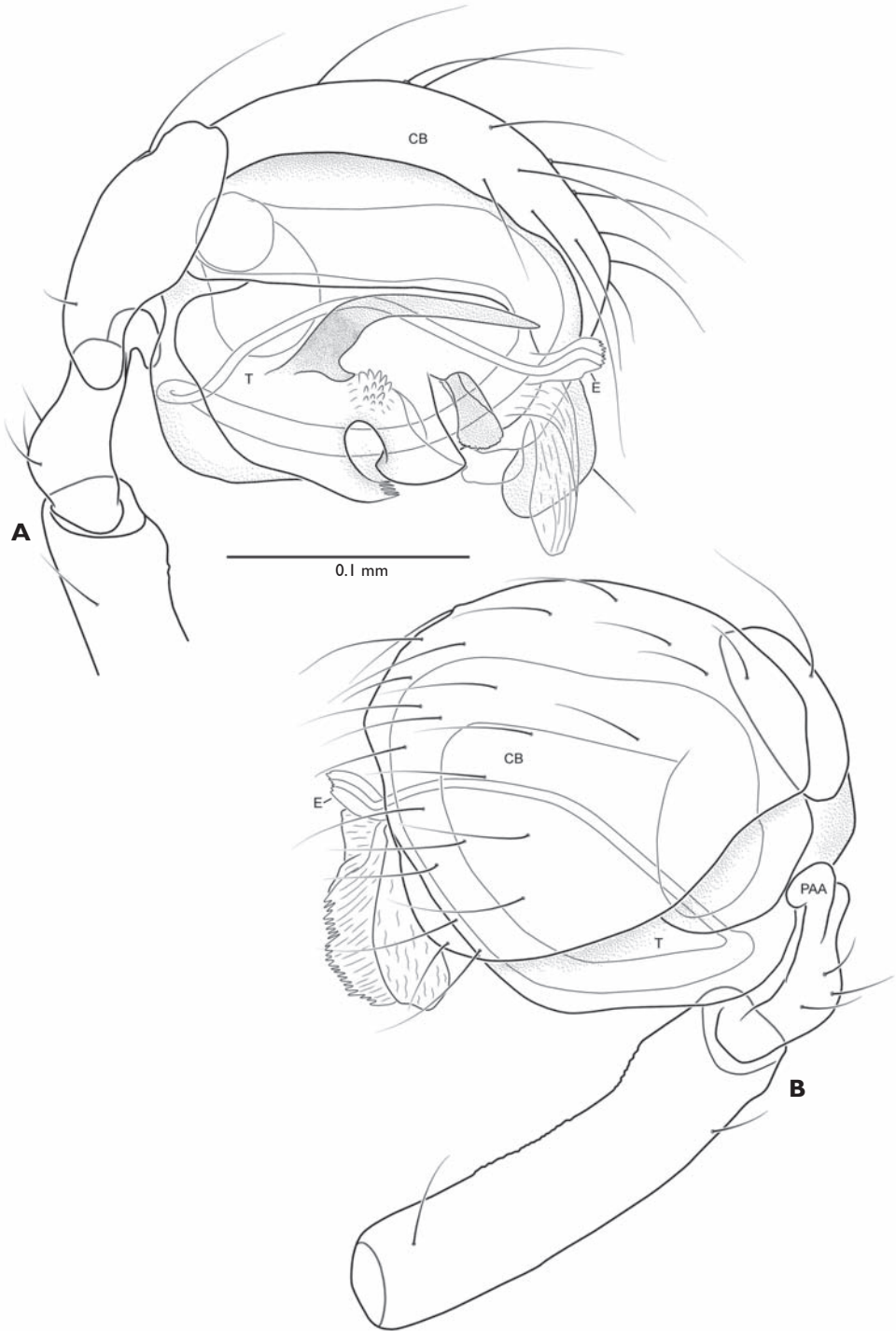
Figure 60. Gaiziapis zhizhuba sp. n. from Nankang Yakou, male palp. A, prolateral; B, retrolateral. CB: cymbium; E: embolus; PAA: patella apophysis; T: tegulum.
