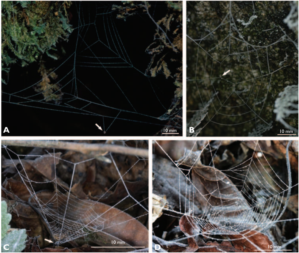
Figure 7. Webs of theridiosomatid spiders. A, Ogulnius barbandrewsi sp. n. from No. 12 Bridge Camp area, juvenile; B, Ogulnius barbandrewsi sp. n. from Guocai He at Fucui, juvenile, arrow to spider facing away from hub, tensing radial thread; C, D, Theridiosoma diwang sp. n. from Xiao Hei Shan Nature Reserve, female. Arrows indicate location of spider.
