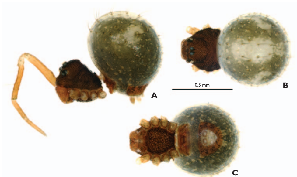
Figure 90. Crassignatha longtou sp. n. from Yamu He, female. A, lateral; B, dorsal; C, ventral.
