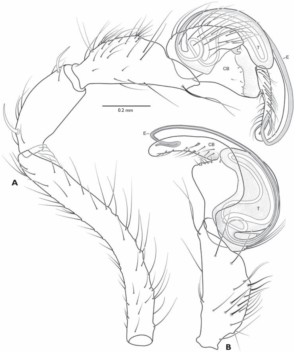
Figure 54. Maymena paquini sp. n. from Wayala Ku cave, male palp. A, prolateral; B, retrolateral. CB: cymbium; E: embolus; T: tegulum.
