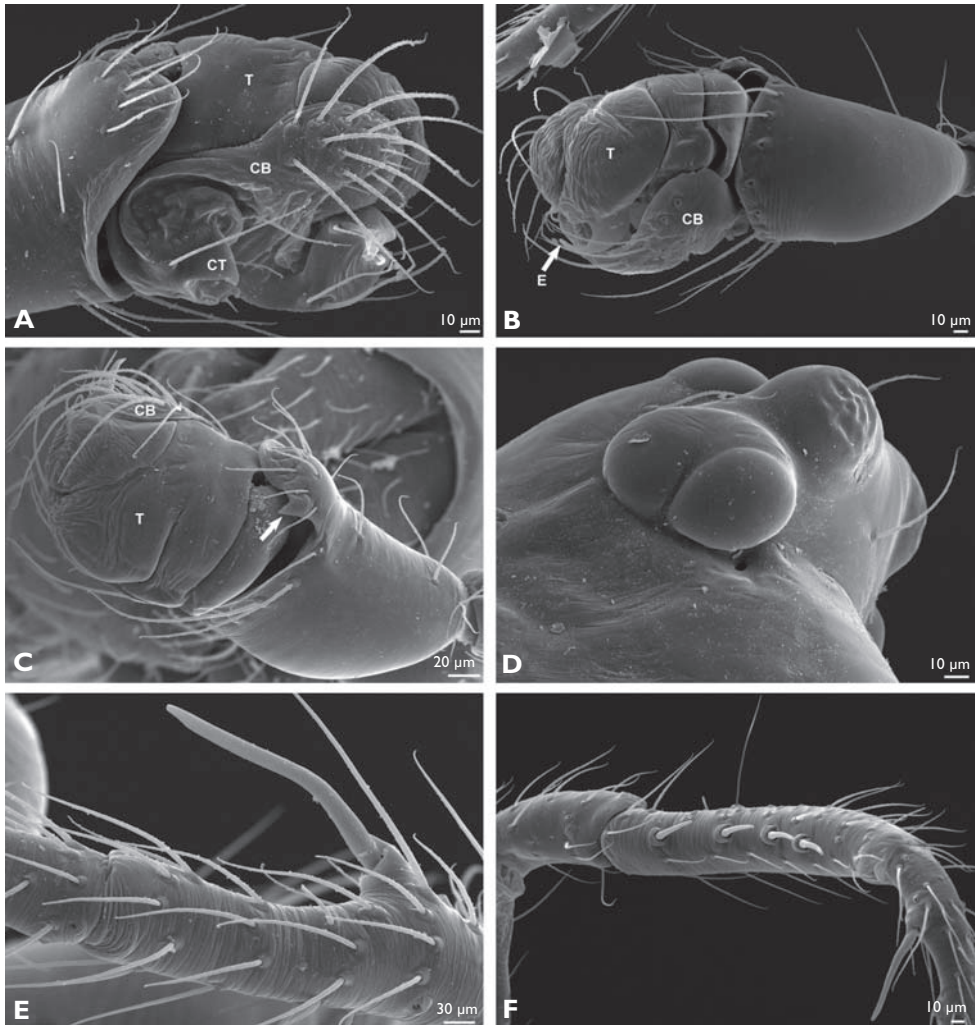
Figure 34. Simaoa yaojia sp. n. from Yaojiaping, SEM of male. A, male palp, prolateral; B, male palp, retrolateral; C, male palp, dorsal, arrow indicates tooth-like tibial process; D, prosoma, anterior lateral; E, metatarsus I; F, tibia I, prolateral. CB: cymbium; CT: cymbial tooth; E: embolus; T: tegulum.
