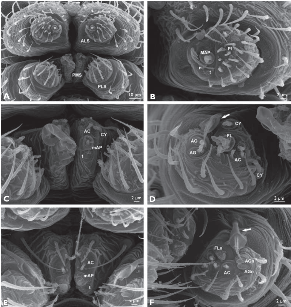
Figure 19. Mysmena changouzi sp. n. from No. 12 Bridge Camp area, SEM of spinnerets. A, female spinnerets; B, female ALS; C, female PMS; D, female PLS; E, male PMS; F, male PLS. AC: aciniform gland spigot; AG: aggregate gland spigot; AGn: aggregate gland spigot nubbin; ALS: anterior lateral spinneret; CY: cylindrical gland spigot; FL: flagelliform gland spigot; FLn: flagelliform gland spigot nubbin; MAP: major ampullate gland spigot; mAP: minor ampullate gland spigot; n: nubbin; PI: piriform gland spigot; PLS: posterior lateral spinneret; PMS: posterior median spinneret; t: tartipore; arrow indicates modified PLS seta.
