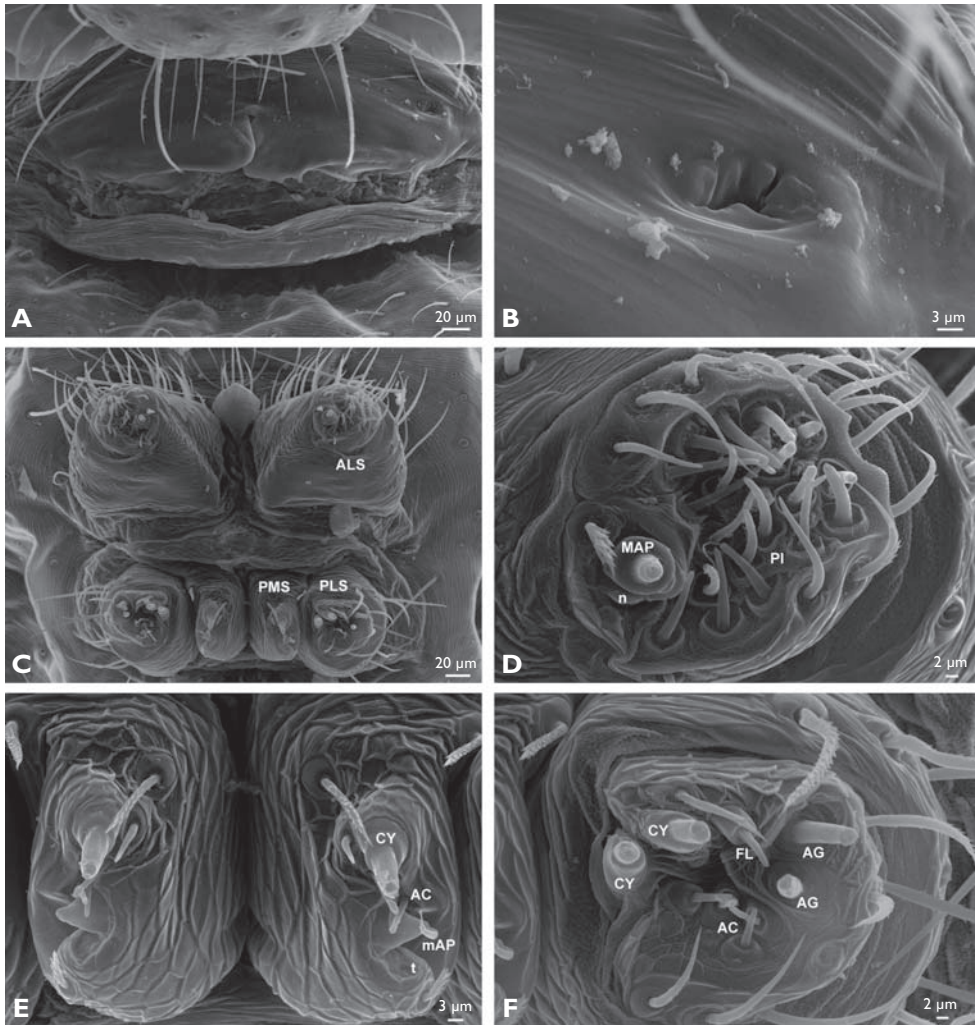
Figure 9. Theridiosoma diwang sp. n. from Xiao Hei Shan Nature Reserve, SEM of female. A, epigynum; B, epigynum, detail showing lateral pore; C, spinnerets; D, ALS; E, PMS; F, PLS. AC: aciniform gland spigot; AG: aggregate gland spigot; CY: cylindrical gland spigot; FL: flagelliform gland spigot; MAP: major ampullate gland spigot; mAP: minor ampullate gland spigot; n: nubbin; PI: piriform gland spigot, PLS: posterior lateral spinneret, PMS: posterior median spinneret, t: tartipore.
