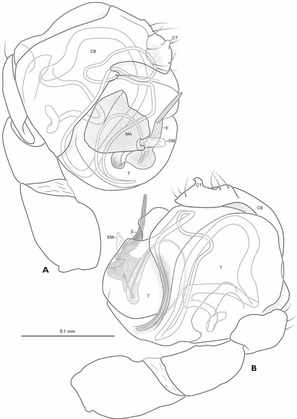
Figure 81. Crassignatha yinzhi from Xiao Hei Shan Nature Reserve, male palp. A, prolateral; B, retrolateral. CB: cymbium; CT: cymbial tooth; E: embolus; EM: embolic membrane; MA: median apophysis; T: tegulum.
