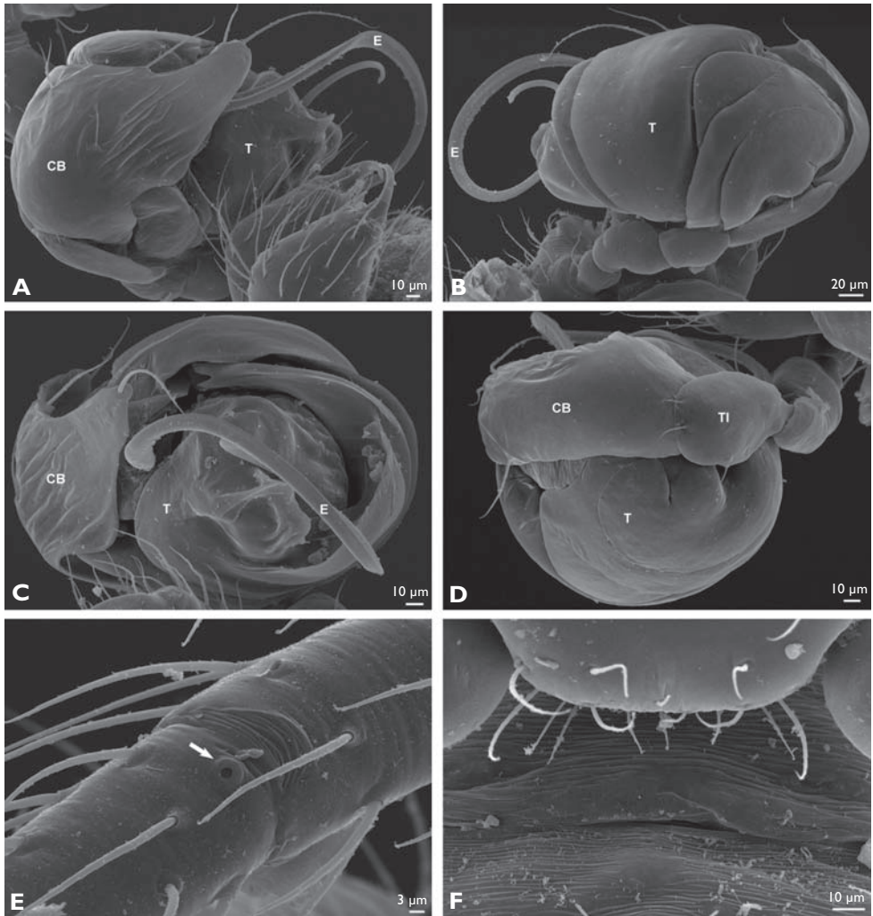
Figure 68. Patu jidanweishi sp. n. from Chang Yan He, SEM of male. A, palp, prolateral; B, palp, retrolateral; C, palp, apical; D, palp, dorsal; E, metatarsus-tarsus joint, arrow indicates tarsal organ; F, epiandrous region. CB: cymbium; E: embolus; T: tegulum; TI, tibia.
