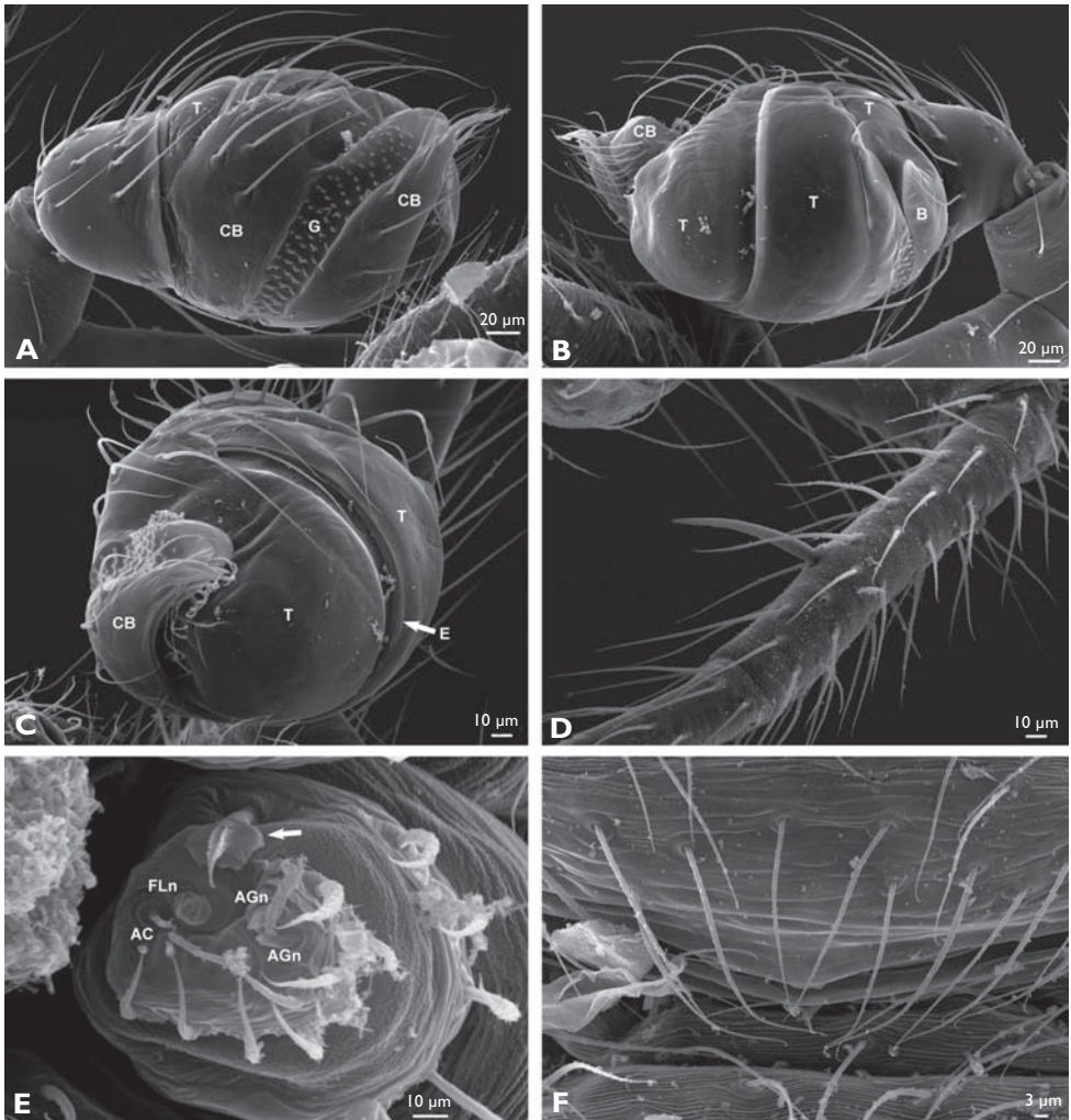
Figure 29. Mysmena goudao sp. n. from QiQi He, SEM. A-E, male; F, female. A, palp, prolateral; B, palp, retrolateral; C, palp, apical; D, metatarsus I; E, PLS, arrow indicates modified PLS seta; F, epigynum. AC: aciniform gland spigot; AGn: aggregate gland spigot nubbin; B: base of cymbium; CB: cymbium; E: embolus; FLn: flagelliform gland spigot nubbin; G: cymbial groove; T: tegulum.
