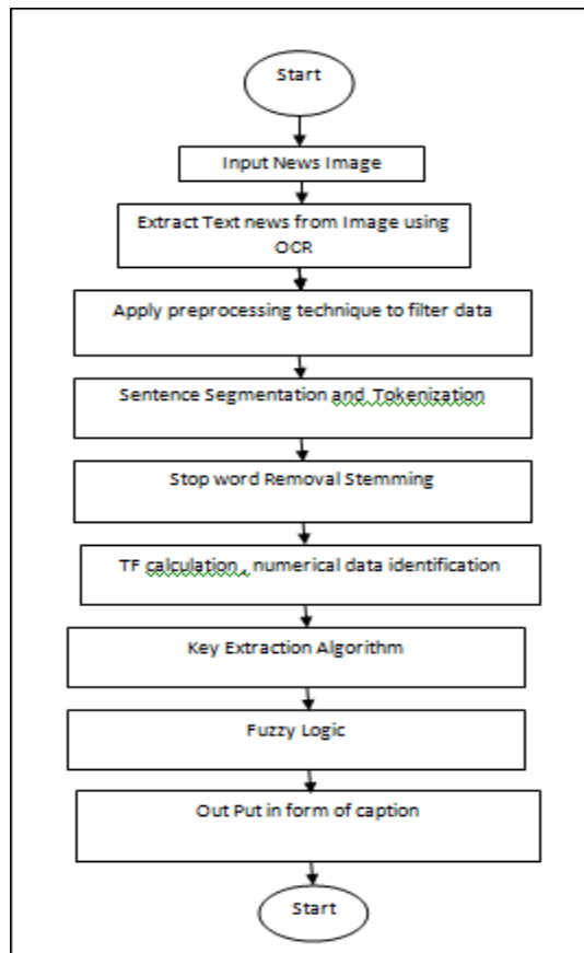
Figure1: Data Flow Dig. For Caption Generation
