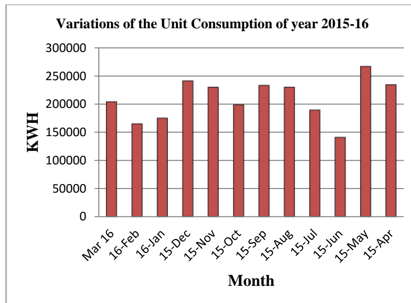
Figure 1- Variation of the unit consumption of year 2015-16
