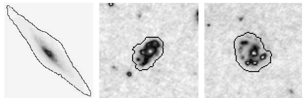
Figure 4: Detection results for NGC 2683, HDF4-378, HDF4-550 (left to right)
