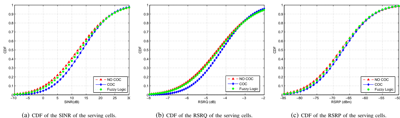
Fig. 11: Comparison of the CDF of SINR, RSRQ and RSRP of the COC with Fuzzy Logic, and NO COC
