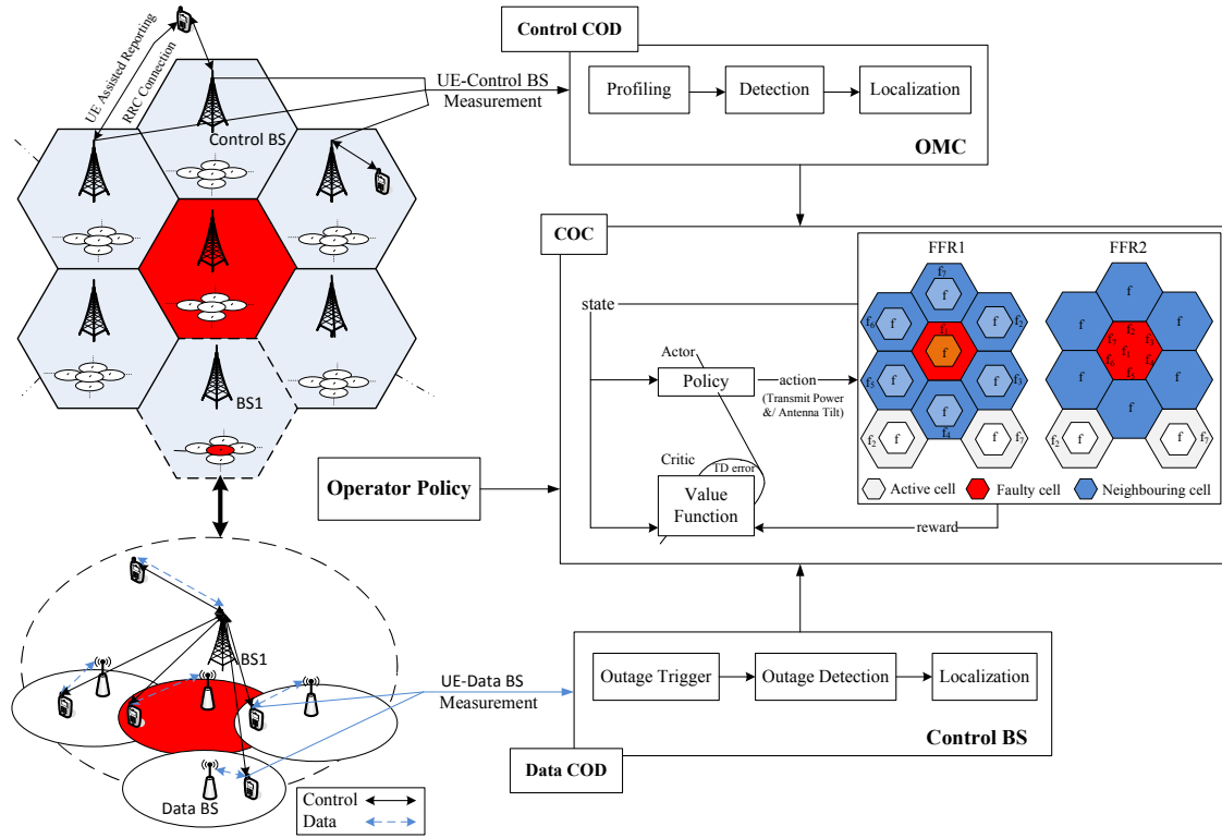
Fig. 1: An overview of COM framework
