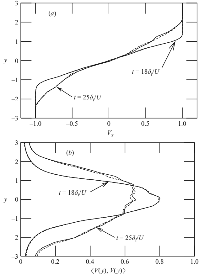
FIGURE 21. Comparison between CVS (dashed line) and DNS (solid line). Cross-stream profile of mean (a) and variance (b) of the streamwise velocity at time t = 18\delta_m^0/\Delta U and t = 25\delta_m^0/\Delta U .
