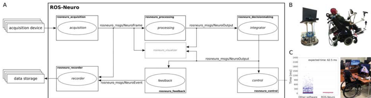
Fig. 1. A) Schematic representation of ROS-Neuro architecture with the available modules and messages. B) BMI driven robotic applications tested with ROS-Neuro. C) On the left, comparison of the data processing delays between ROS-Neuro and previous validated BMI software; on the right, the use of a BMI system implemented in ROS-Neuro during the Cybathlon 2020 event.
