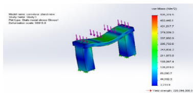
Fig. 6 Stress Analysis of stand.
