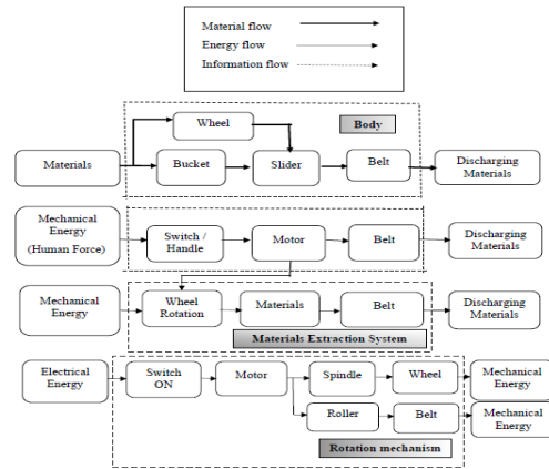
Fig. 2 The Cluster Function Structure
