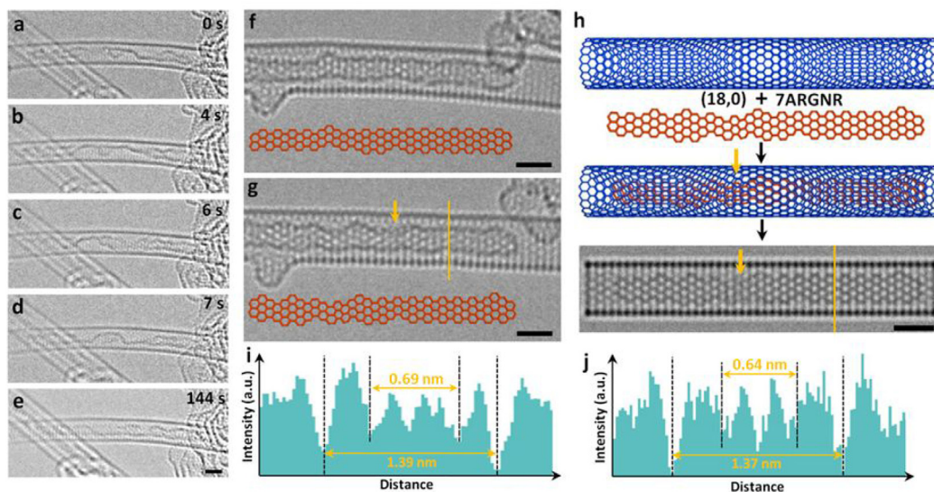
Fig. 1. AC-HRTEM images and corresponding simulations for AGNR@SWCNTs. a–e, Time series of images showing a ribbon confined in a SWCNT twisting under 80 keV electron beam. The modulation of the response with time is evidence for a flat ribbon. f, g, Two typical AC-HRTEM images in atomic resolution showing a flat 7-AGNR dominated structure confined in a SWNT. Scale bar is 1 nm. The inserted models in red present the corresponding structure of the ribbon, showing also the instability of the ribbon under electron beam irradiation (i.e., f–g are the same ribbon but acquired after different exposure times). h, TEM image simulation for confirming the structure of 7-AGNR@SWCNT in g. It depicts the tube (18,0), the ribbon, the combination of the two and the simulation. The most part of 7-AGNR and the wall of SWNT are AA stacked showing clear graphene structure for the former, while a small mismatch part as indicated by yellow arrows results in blurred contrast in the simulated TEM and in the raw TEM image in g. i, j, Intensity profiles along the yellow line of the recorded pattern i and of the simulated pattern j. The round (outer) tubes exhibit a strong reduction of contrast at the edge whereas the contrast is weaker at the edge of the flat ribbons. Indicated distances correlate with the diameter of a (18,0) tube and evidence a net ribbon width between 0.64 and 0.69 nm. (A colour version of this figure can be viewed online.)
