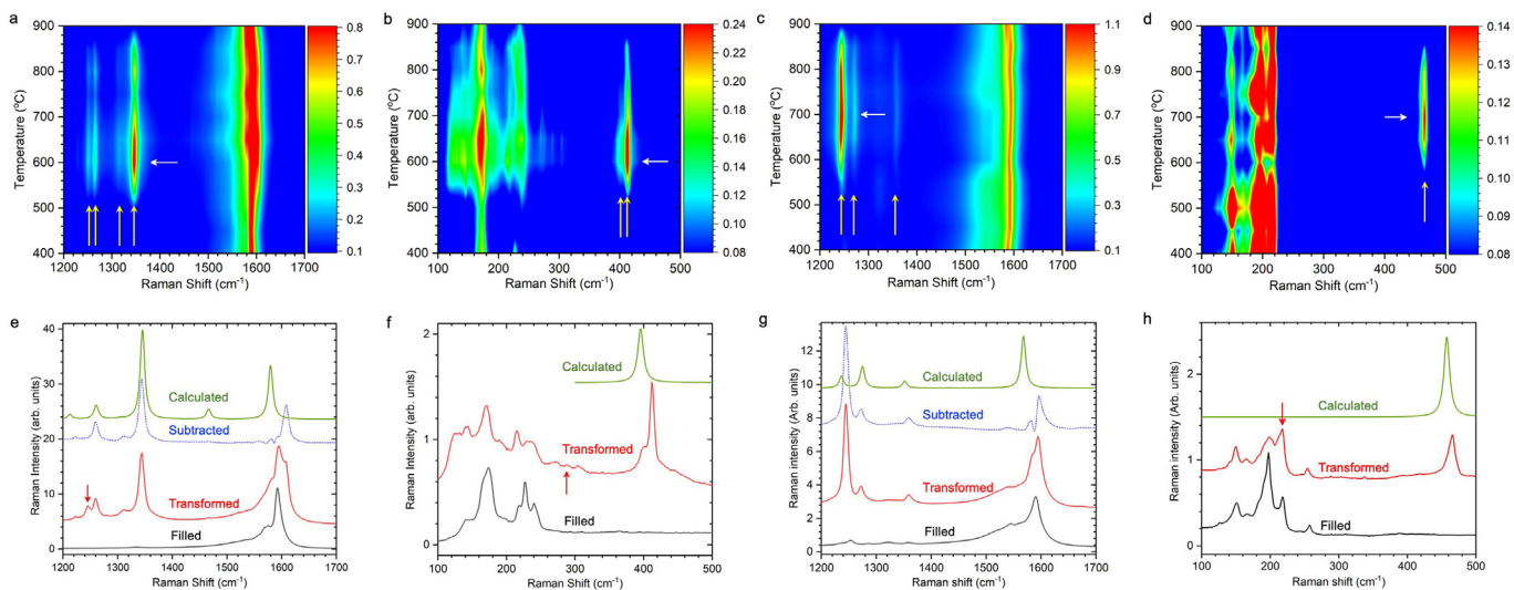
Fig. 2. Raman scattering for temperature dependent transformation. a–d, Color-code maps for Raman line intensities observed after transformation of FeCp 2 @SWCNTs as a function of Raman frequency and transformation temperature. The latter was increased in 50 °C steps. Vertical white arrows highlight the positions of the main new Raman lines. Horizontal white arrows are located at temperatures of maximum Raman response. Raman spectra in a and b and in c and d were excited with a yellow laser (568 nm) and red laser (633 nm), respectively. e–h, Raman spectra for FeCp 2 @SWCNT tuned by transformation temperature to optimized response for the two groups of lines. e, Spectra as observed for yellow laser excitation at 568 nm in the high frequency region, from bottom to top: tubes filled with FeCp 2 (black) and subsequent transformation at 600 °C (red), AGNR contribution by subtracting the Raman signals from the nanotubes (blue, dotted), and calculation (green) for 7-AGNR. The Raman line marked by a down-arrow was also subtracted since it originates from 6-AGNR as discussed below. f, Raman signals from low frequency region, from bottom to top: filled tubes, transformed at 600 °C, and calculated for 7-AGNR. The arrow marks the response from DWCNTs obtained during the transformation process. g, h, Similar spectra as in e, f but for transformation temperatures of 700 °C, recorded with 633 nm laser, and as calculated for 6-AGNR. (A colour version of this figure can be viewed online.)
