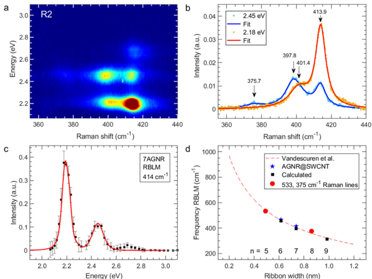
Fig. 4. Raman scattering for the RBLM of 7-AGNR. a, Blown up Raman map for the frequency region between 350 and 440 \text{cm}^{-1} ; b, Radial breathing like mode for 7-AGNR as excited with laser lines at 2.45 (blue) and 2.18 eV (red). Full drawn lines are fits from the experimental analysis. c, Resonance profile for the main peak of the RBLM at 414 \text{cm}^{-1} (dots, with errorbars) together with the calculated values (red line); d, RBLMs frequencies versus ribbon width w . Blue stars are the experimental results from this work. Black squares are calculated values. The dashed line corresponds to Vandescuren et al. [20] who found a relation of the form \omega_{\text{RBLM}} = a/\sqrt{w} - b with empirical parameters a and b for the dependence of the RBLM frequency on w , the ribbon width without hydrogen. The dashed line in the figure was evaluated for a and b equal to 527.4 and 210.2, respectively. Red dots are for the additional Raman lines at 533 and 375 \text{cm}^{-1} if they are assigned to 5-AGNR and 8-AGNR, respectively. The value for n = 9 is from a reference. [7].
