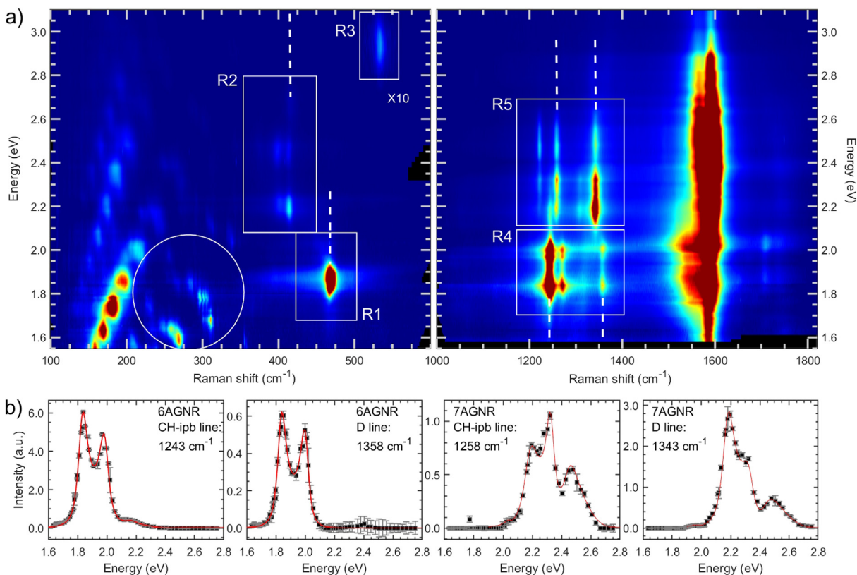
Fig. 3. Wavelength-dependent Raman spectroscopy of AGNR@SWCNT. a, Two-dimensional Raman map for the resonance excitation of AGNR@SWCNT. The features from the ribbons are framed into the white rectangles with numbers R1 to R5. The rectangles R2 and R5 correspond to the 7-AGNR whereas rectangles R1 and R4 correspond to the 6-AGNR. R3 (intensity multiplied by 10) most likely originates from 5-AGNR (see below). The bulky feature around 1600 cm -1 comes mainly from a superposition of the G line of the nanotubes and the AGNR. The circled signals originate from double-walled carbon nanotubes grown during transformation. They correspond to the weak Raman lines in Fig. 2e and f assigned by the arrows. b, Experimental Raman excitation profiles derived for the Raman peaks that are indicated by the dashed white lines in panel a are presented as black squares together with the fitted Raman excitation profiles (in red) for the 6-AGNR (left) and 7-AGNR (right) (See also Supporting Information section (e)). The profiles correspond to the CH-ipb and D -line, respectively. (A colour version of this figure can be viewed online.)
